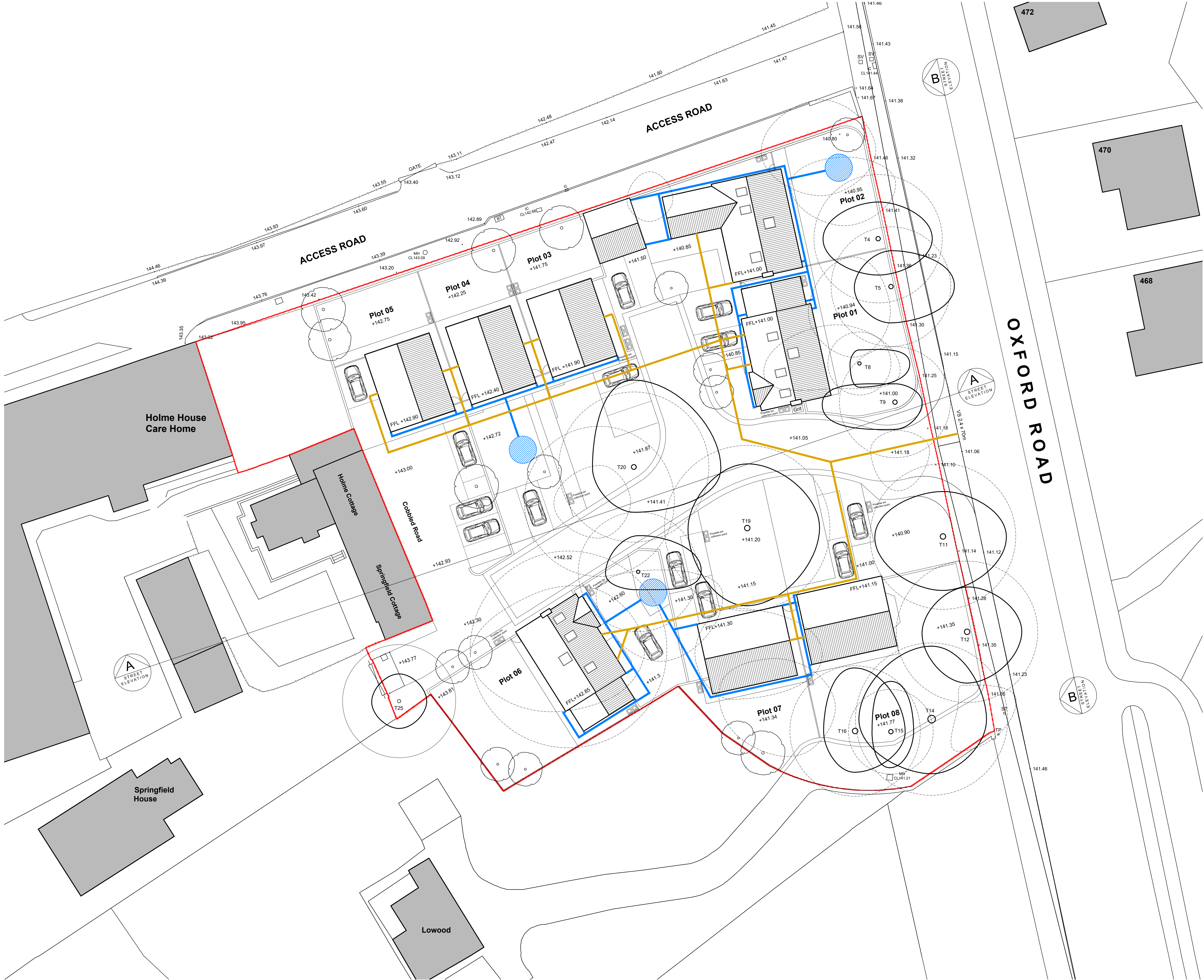
INDICATIVE DRAINAGE LAYOUT 1:200 @ A1
