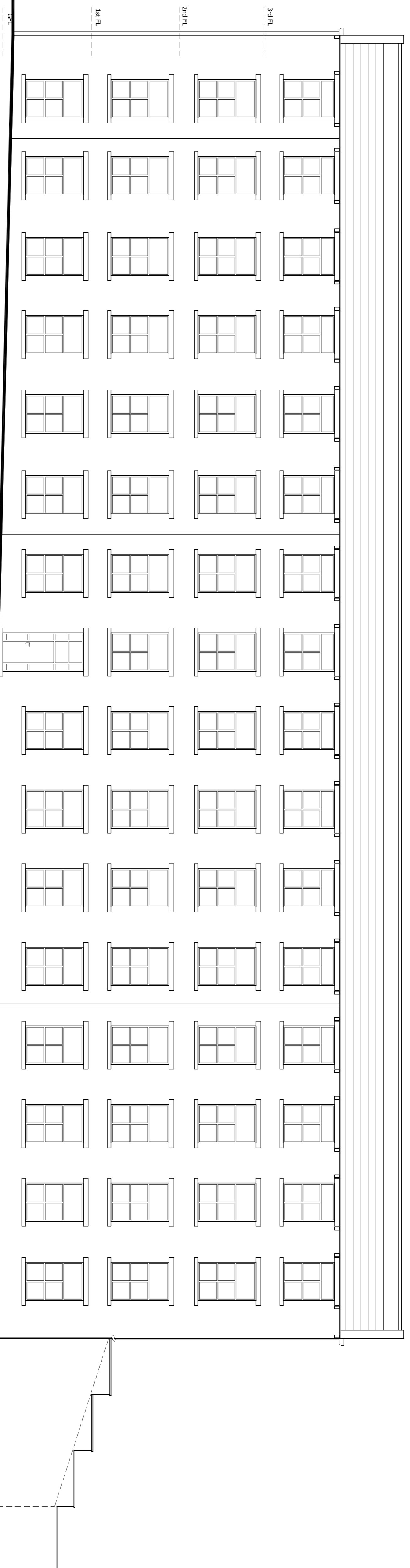
Front Elevation as Existing
