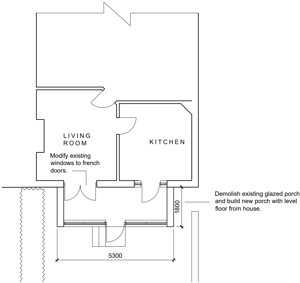
PROPOSED CONSERVATORY FLOOR PLAN 1:100
