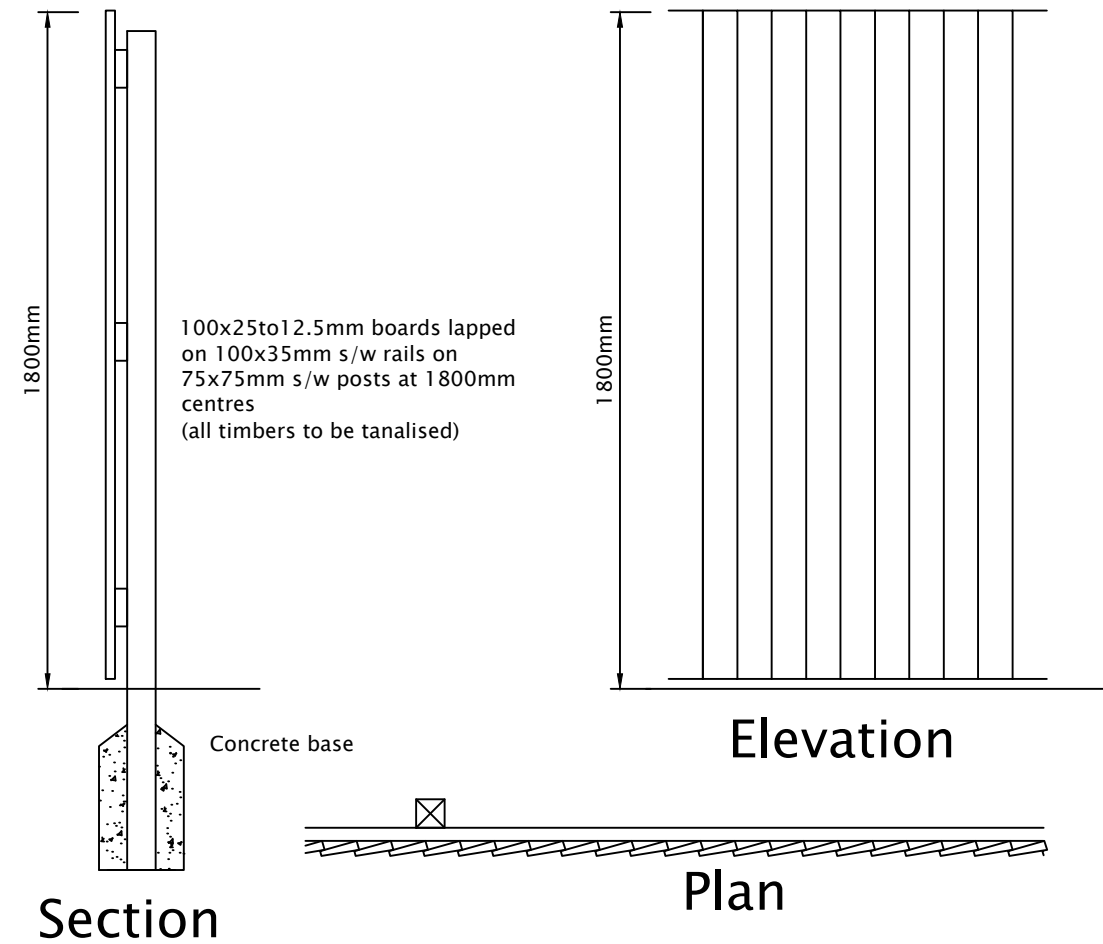
Lap boarded timber fence 1800mm high
