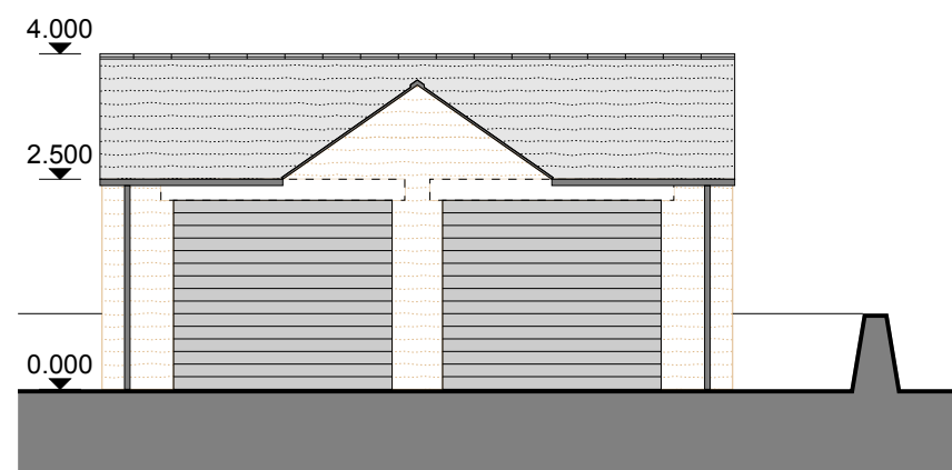
WEST ELEVATION - 1:100
