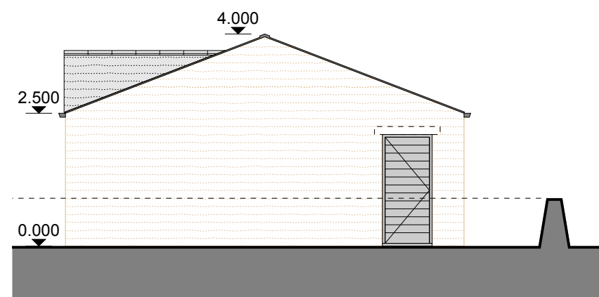
SOUTH ELEVATION - 1:100
