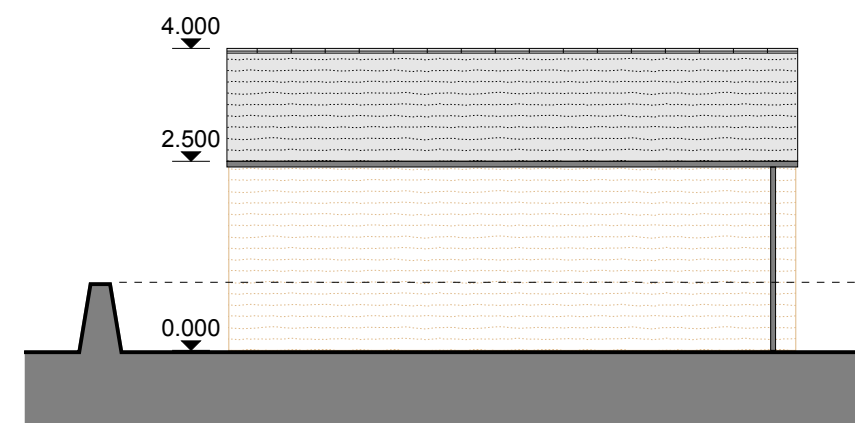
EAST ELEVATION - 1:100
