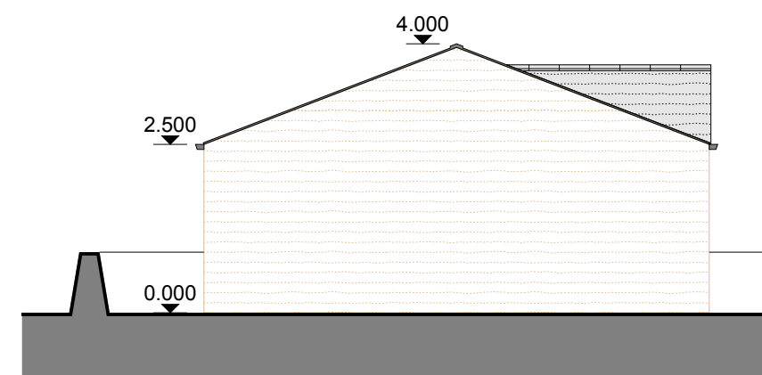
NORTH ELEVATION - 1:100
