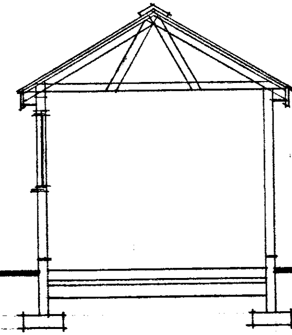
SECTION
