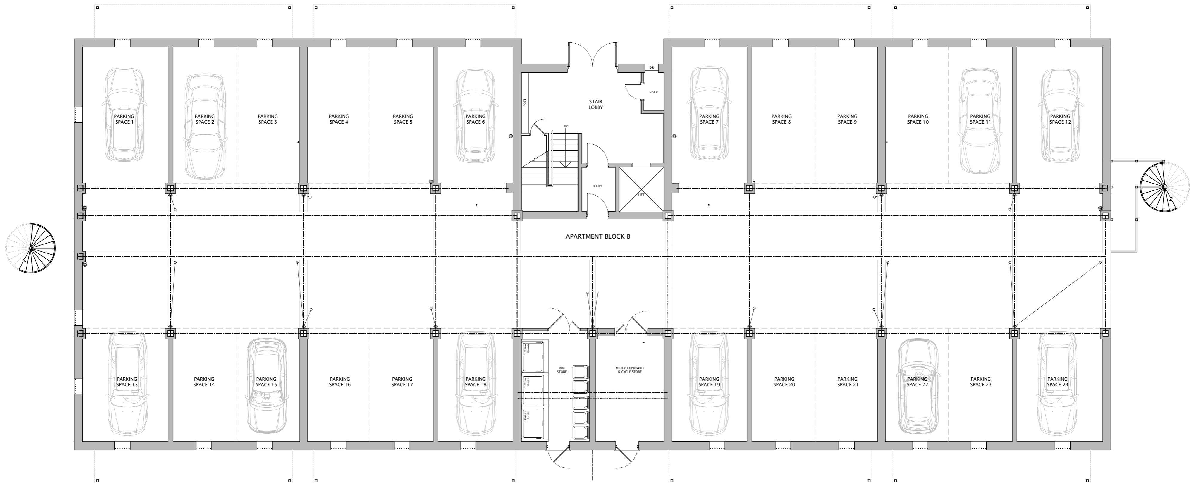
GROUND FLOOR LAYOUT
