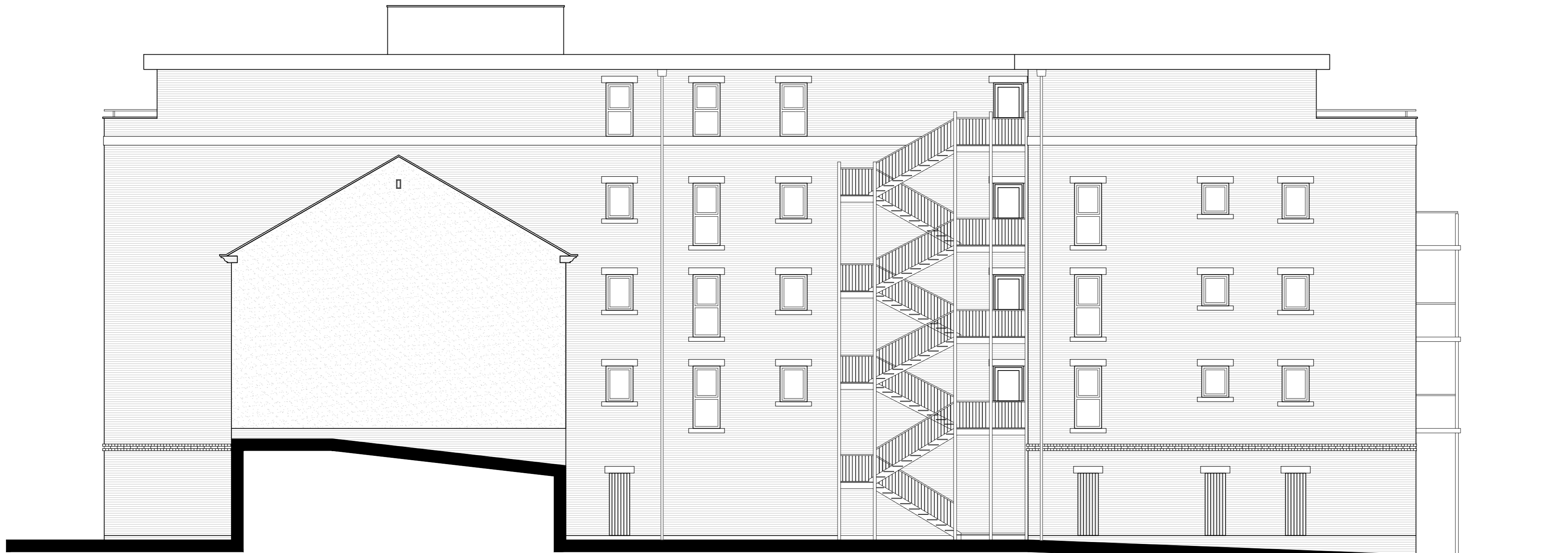
NORTH ELEVATION
