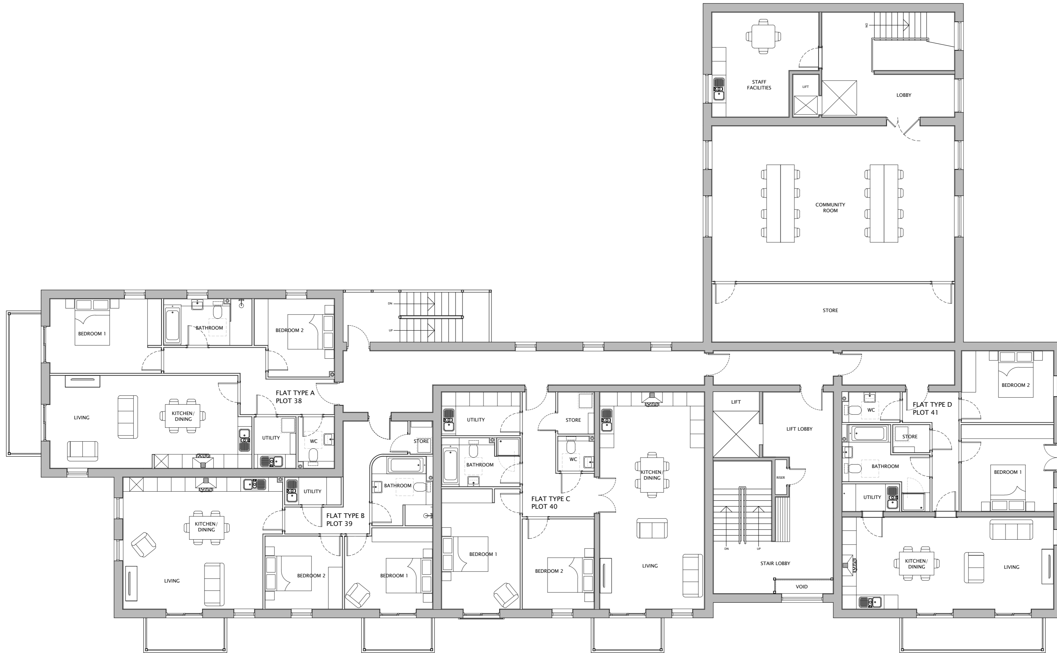
SECOND FLOOR LAYOUT
