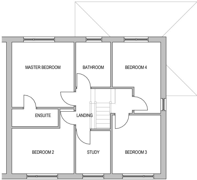
FIRST FLOOR - PROPOSED 1 : 100
