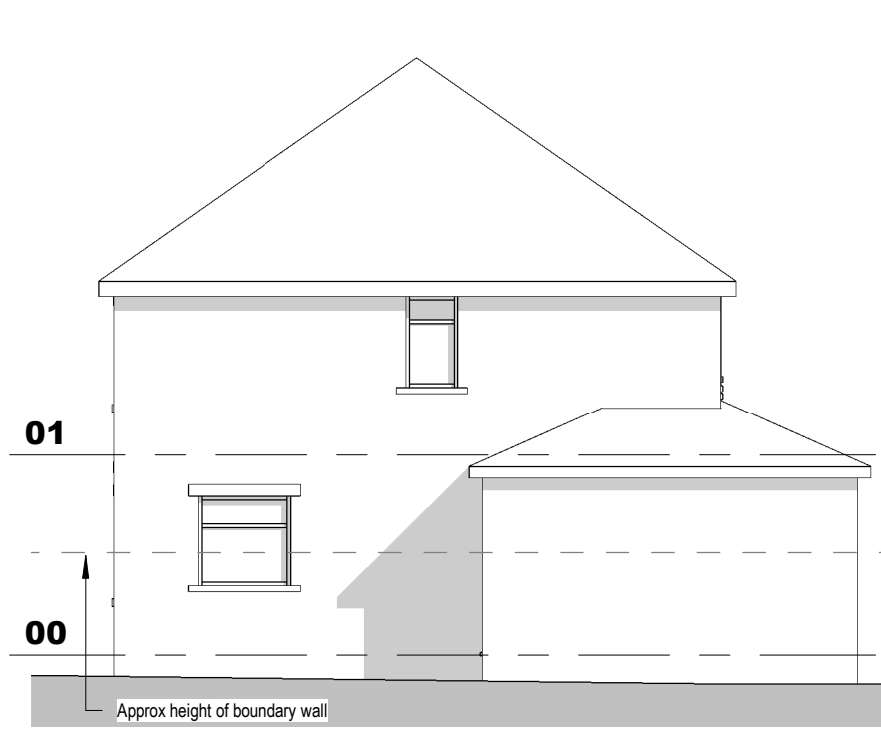
SIDE ELEVATION 1 1 : 100
