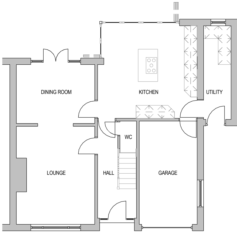
GROUND FLOOR - PROPOSED 1 : 100
