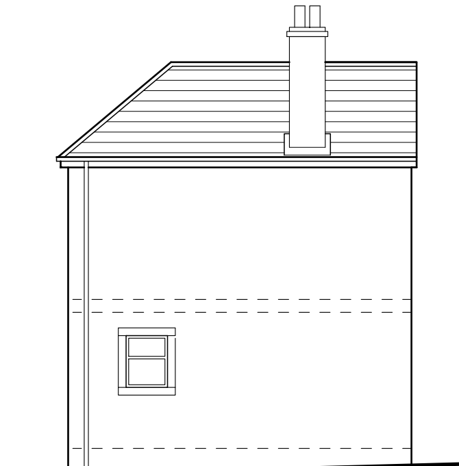
side elevation
