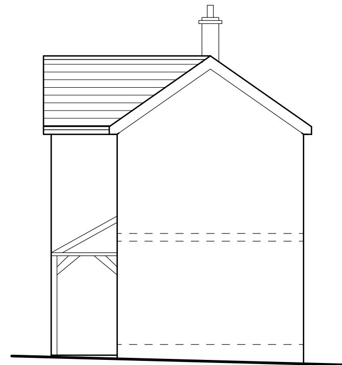
gable elevation
