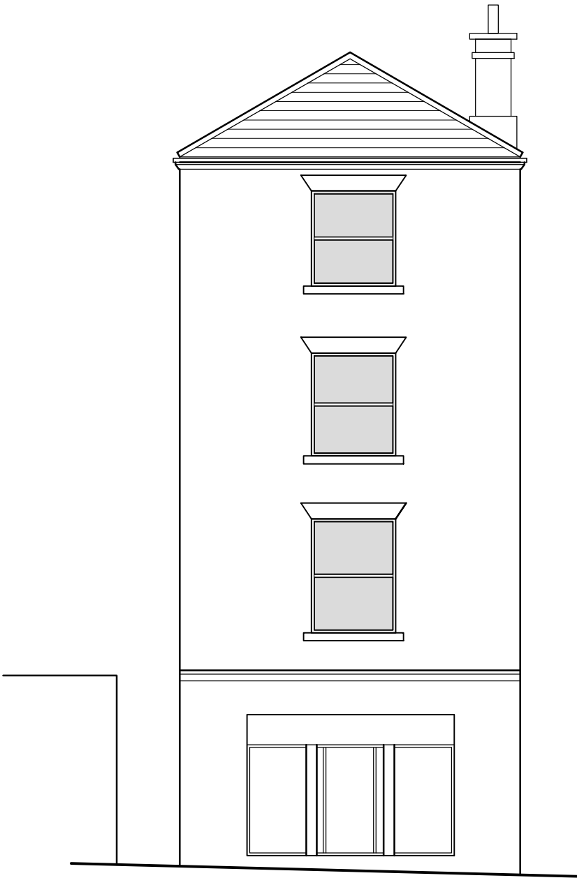
FRONT ELEVATION - EXISTING 1:100
