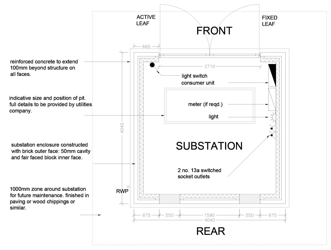
1 Substation Layout 1:50
