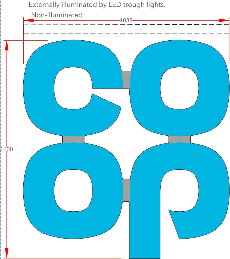
1100mm Scale 1:10 @A3
