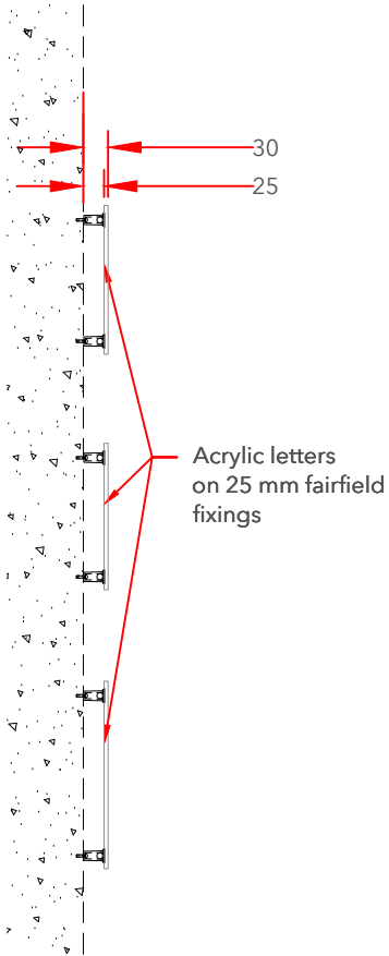
Letters Cross Section Scale 1:10 @A3
