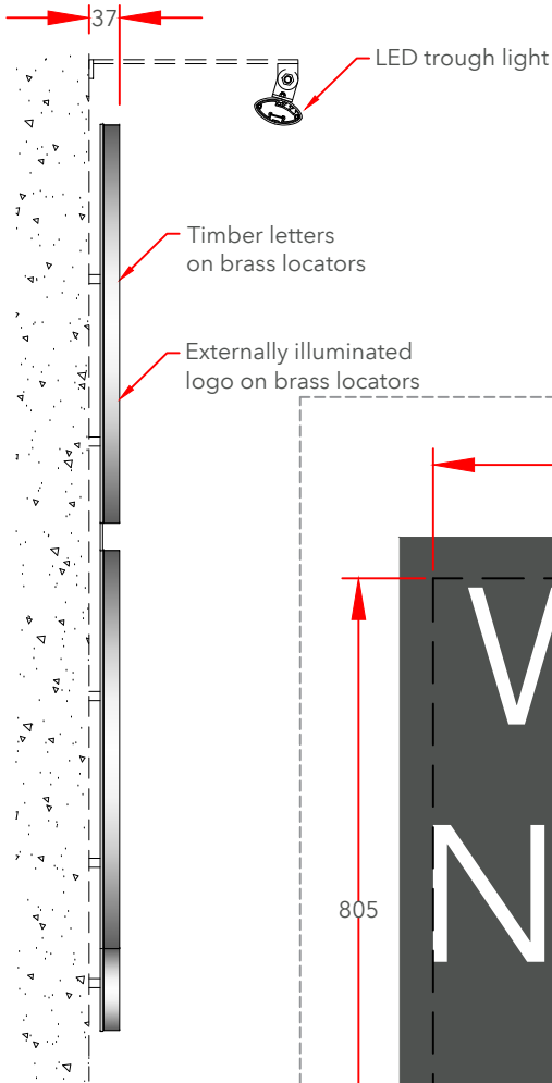
Cross Section Scale 1:10 @A3
