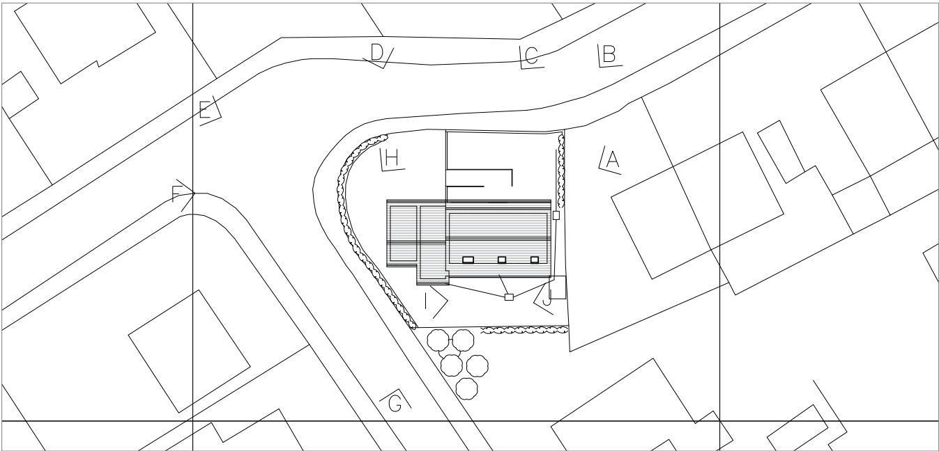
KEY PLAN 1:500
