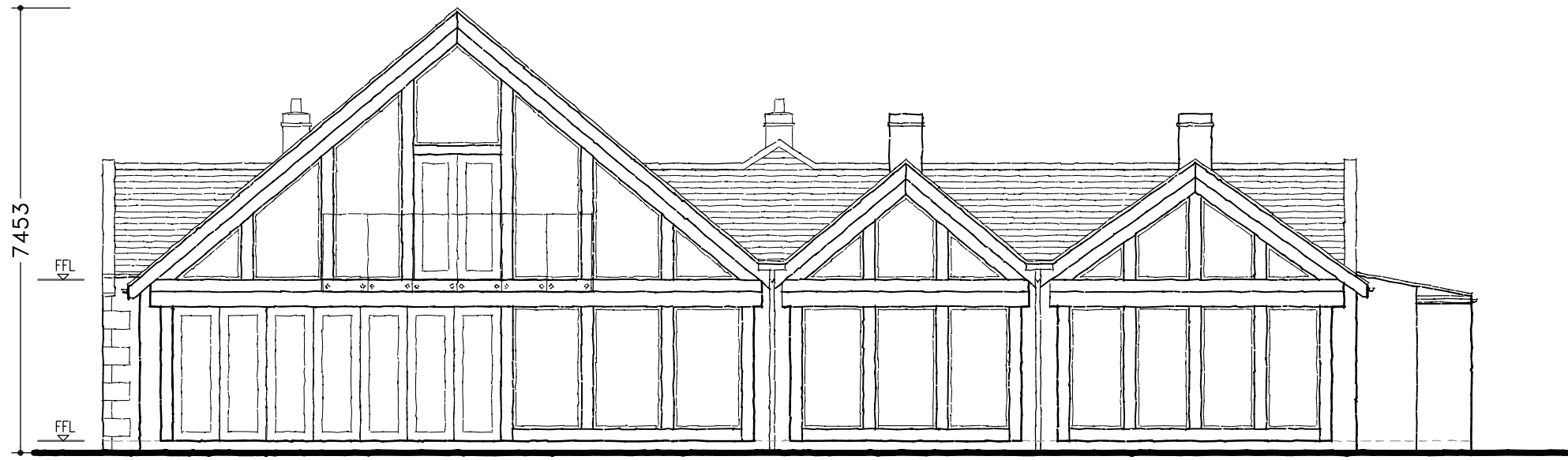
SOUTH ELEVATION
