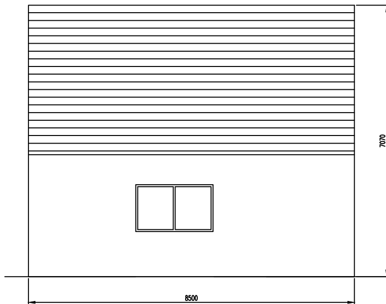
NORTH ELEVATION
