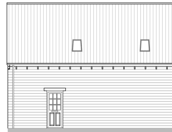
REAR ELEVATION PLOT 1 and 4
