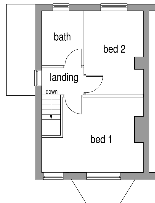
Existing first floor layout (1:100)
