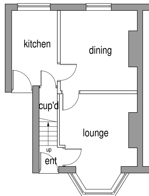
Existing ground floor layout (1:100)
