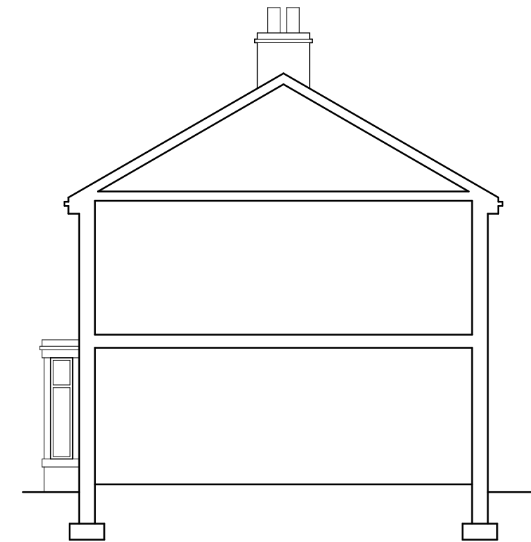
Existing sectional elevation (1:100)
