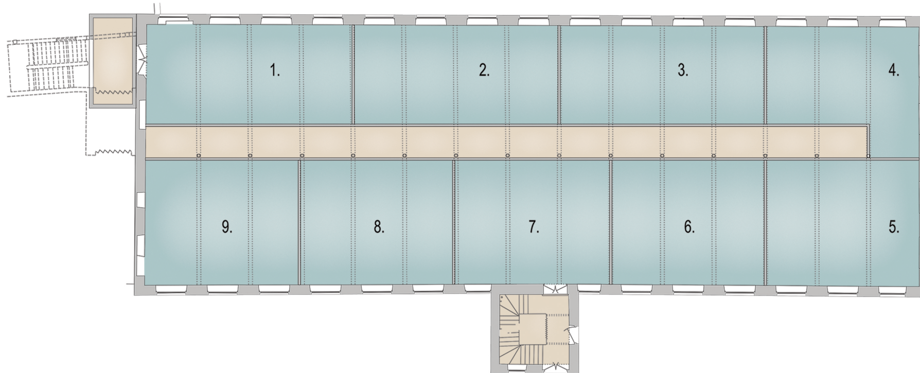
Indicative Floor Plan Third Floor Possible Uses: Residential C3 Max 18No. Units between Second & Third Floor
