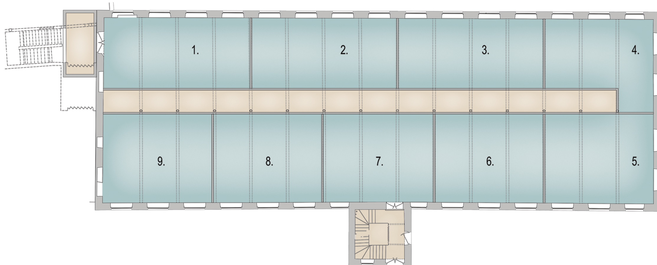
Indicative Floor Plan Second & Third Floors Possible Uses: Residential C3 Max 18No. Units
