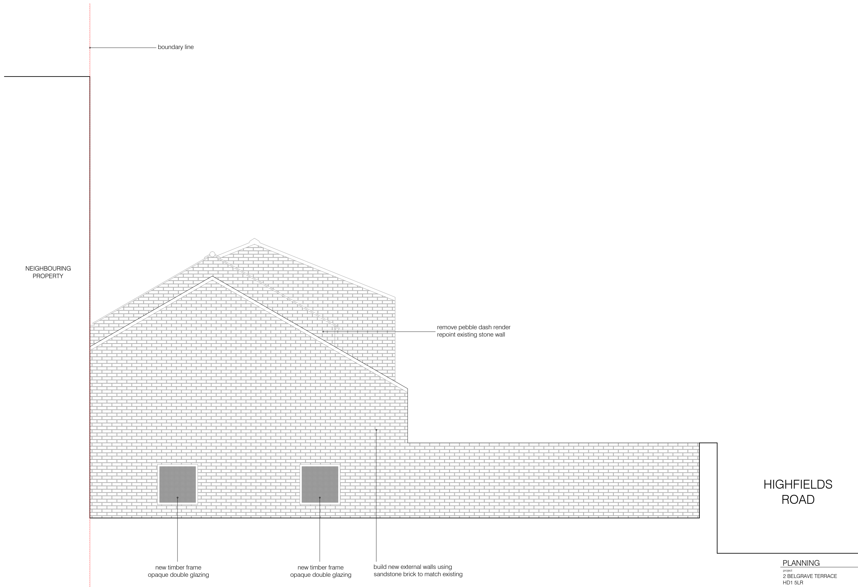
01 PROPOSED SIDE ELEVATION scale 1:50
