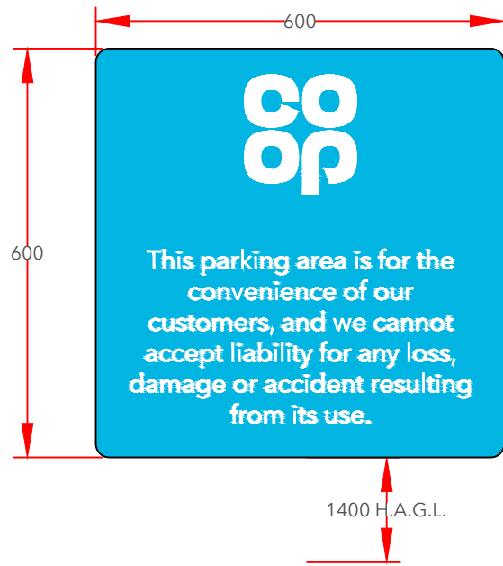
Signs H1, H2 & H3 - Scale 1:10
