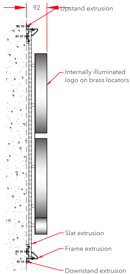
Logo Cross Section Scale 1:10 @A3
