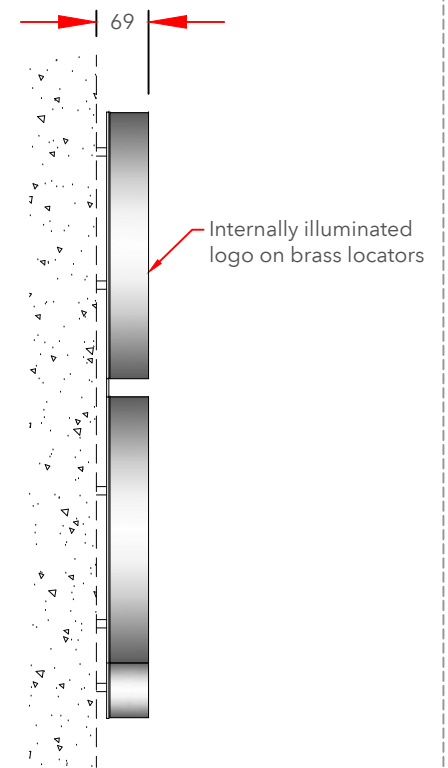
Cross Section Scale 1:10 @A3
