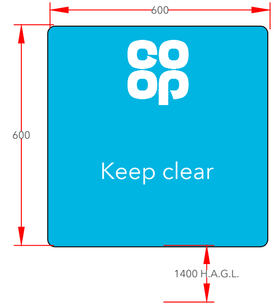
Sign K - Scale 1:10
