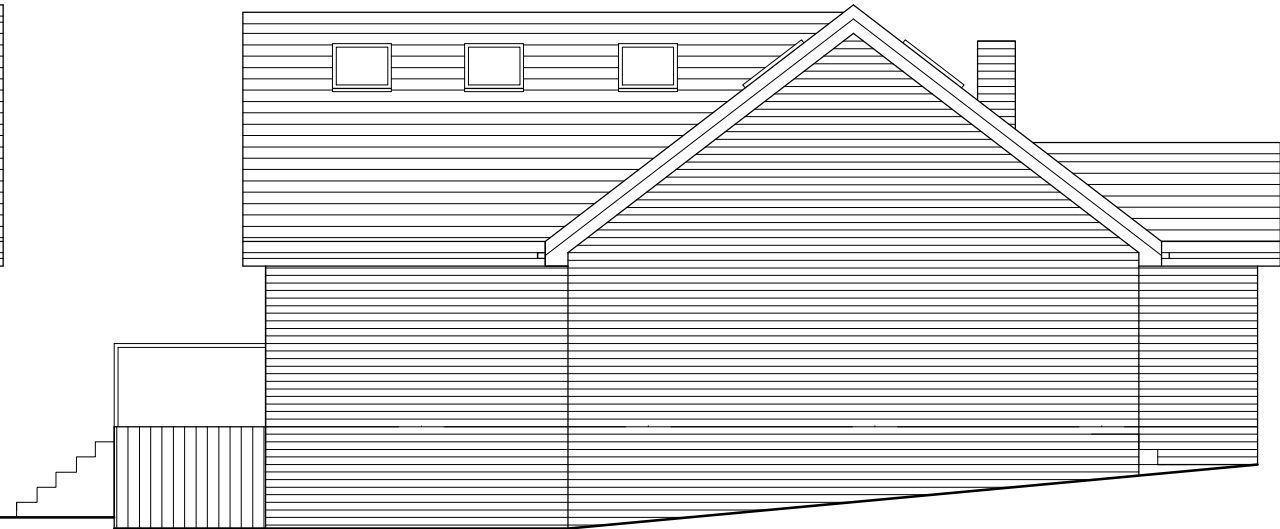
Side Elevation
