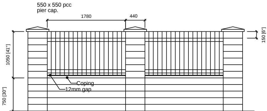
SF1 ARTSTONE WALL AND TIMBER SCREEN 440 x 440 x 1800mm high Artstone piers built off 21N concrete foundations. Depth of foundations to be 750mm minimum below ground level. Walls to be thick (215mm), to be built off 21N concrete strip footing. Copings to be pcc with 50mm overhang all-round, with a 6 x 6mm drip. DPC under any joints. Panels to be 100 x 25mm feather edge boards (20mm lap) fixed to 75x50mm SW runners all preservative stained. All fixings to be galvanised mild steel.
