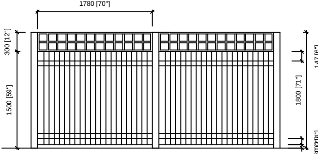
JHYSF12 FEATHER EDGED SCREEN WITH TRELLIS TOP 100x100mm timber posts with 75x50 SW runners (3No.) and 100x25mm thick feather edge boards. Bottom edge of boards to be set 50mm above finished ground level. All to receive preservative stain finish, colour dark brown. Fixings to be galvanised mild steel. Posts to be taken down 600mm minimum and encased centrally in 450x450x600mm deep concrete base.
