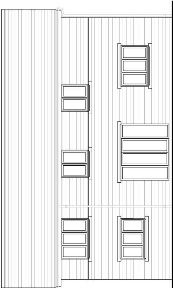
REAR ELEVATION
