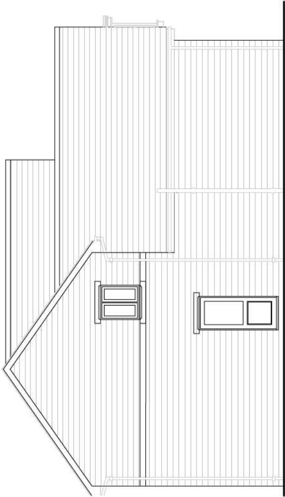
SIDE ELEVATION
