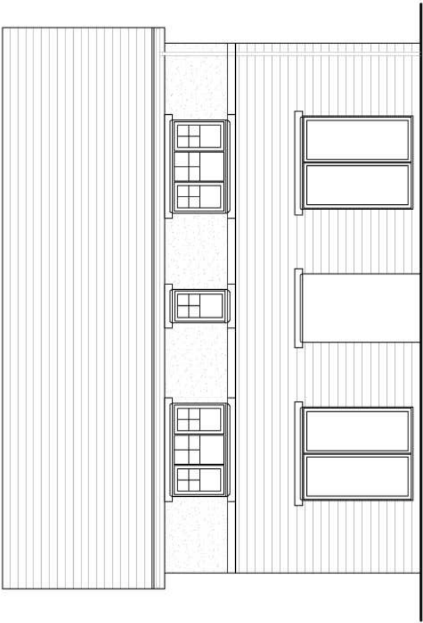
REAR ELEVATION
