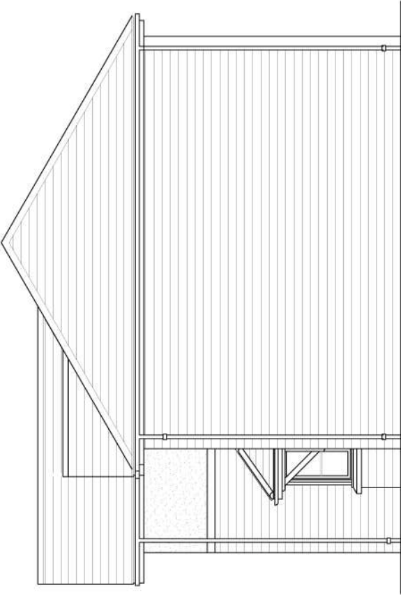
SIDE ELEVATION 1
