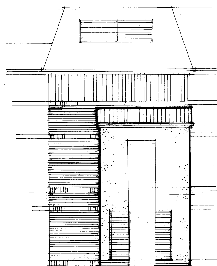
proposed front elevation 1:100
