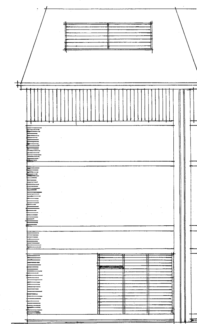
existing elevation 1:100
