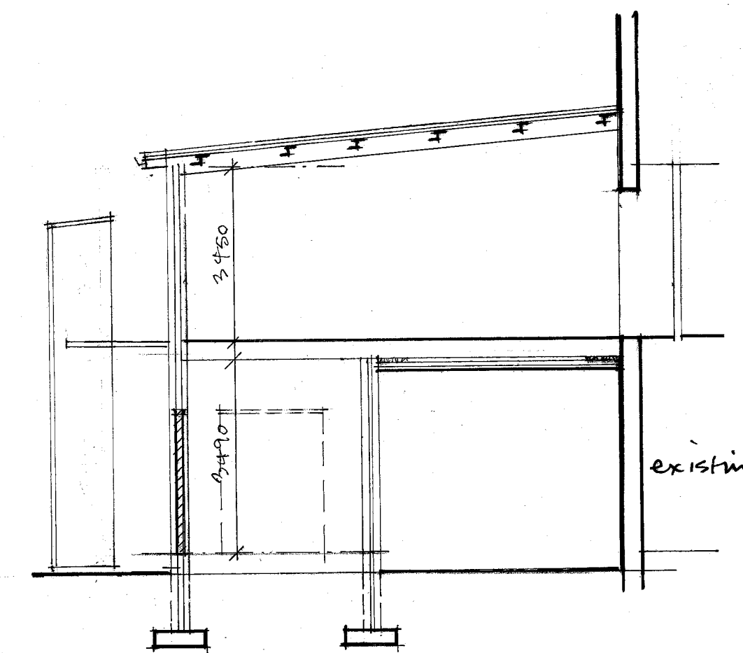
proposed section 1:100
