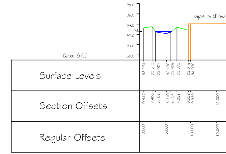
Cross Section 16 HECRAS XS: 28
