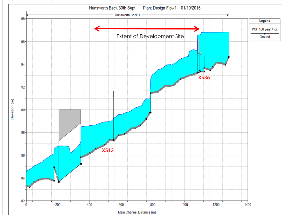
Figure 3.5: Long Section of Hunsworth Beck
