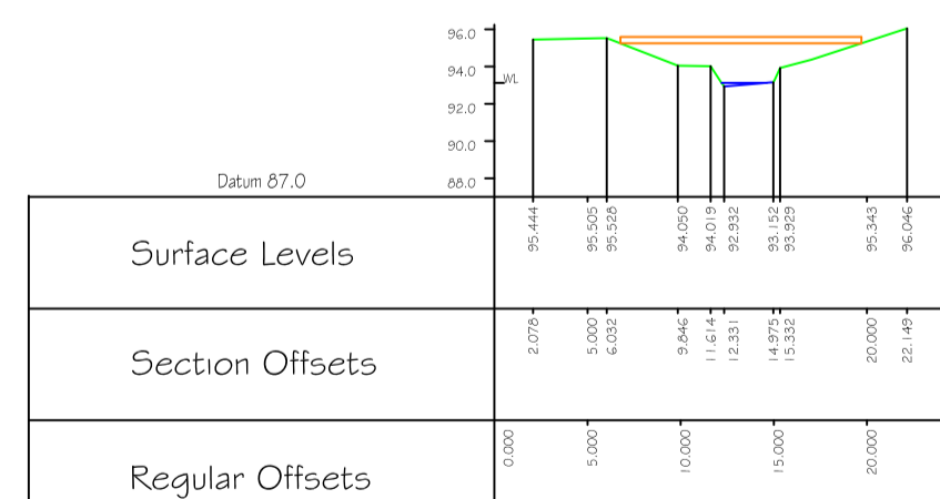
Cross Section 13 HECRAS XS: 31 Derelict Bridge Downstream of section
