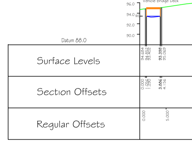
Cross Section 10 HECRAS XS: 34 Culvert face - downstream face, facing downstream
