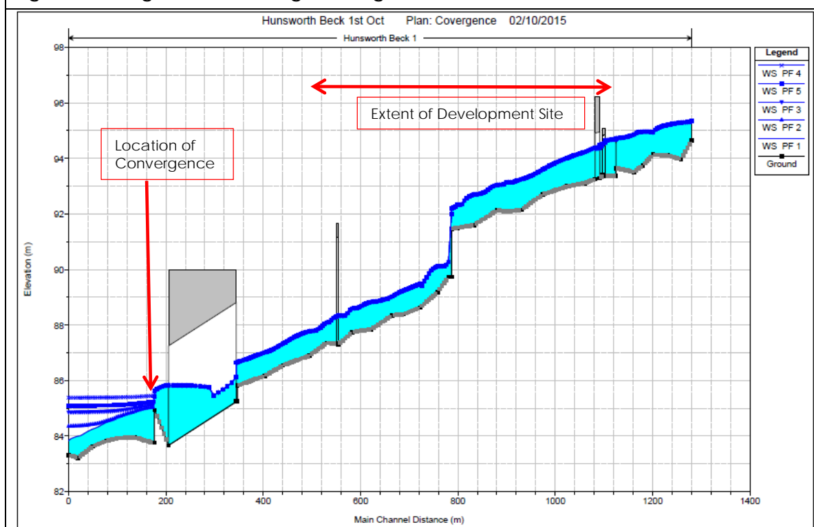
Figure 3.6: Long Section showing Convergence of Flow at weir
