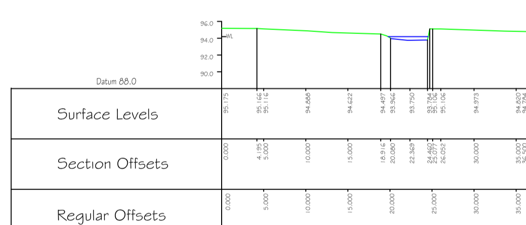
Cross Section 6 HECRAS XS: 38
