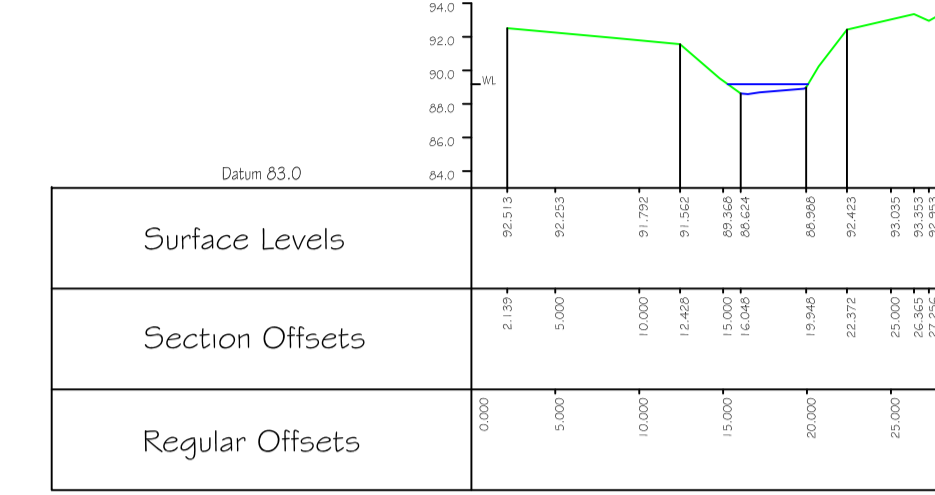
Cross Section 24 HECRAS XS: 20
