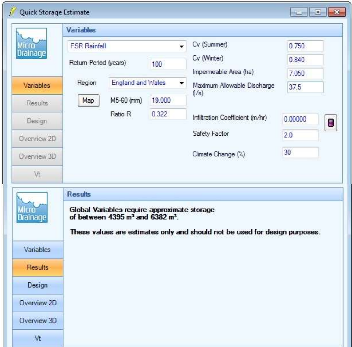
Figure 9. Microdrainage Quick Storage Estimate Attenuation Assessment – Commercial Area B South
