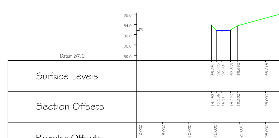
Cross Section 14 HECRAS XS: 30
