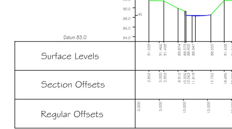
Cross Section 26 HECRAS XS: 18
