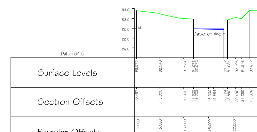
Cross Section 21 HECRAS XS: 23
