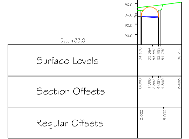
Cross Section 11 HECRAS XS: 33 Culvert face - upstream face, facing downstream
