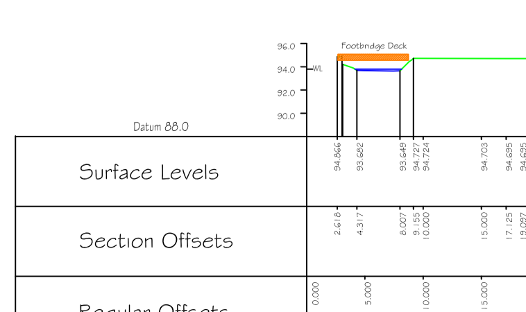
Cross Section 7 HECRAS XS: 37
