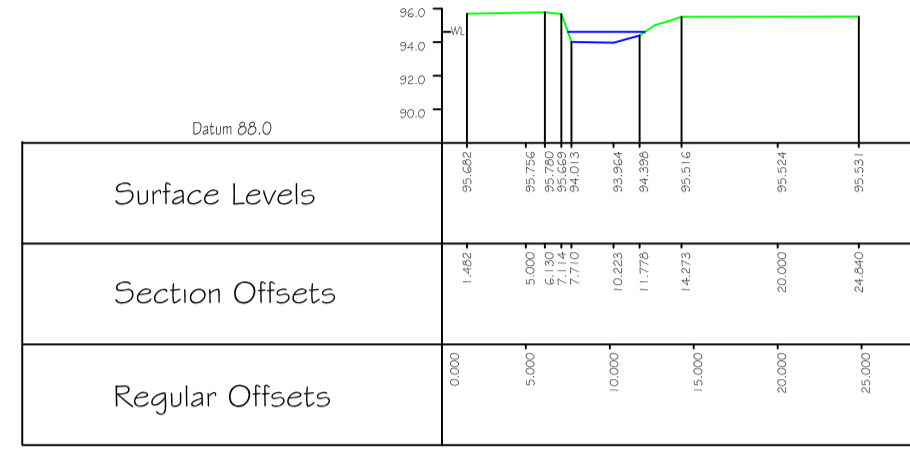
Cross Section 3 HECRAS XS: 41
