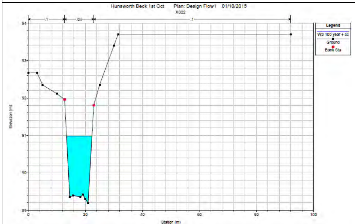
Figure 3.3: Cross Section 22 – 1 in 100 year plus climate change Unobstructed Flow
