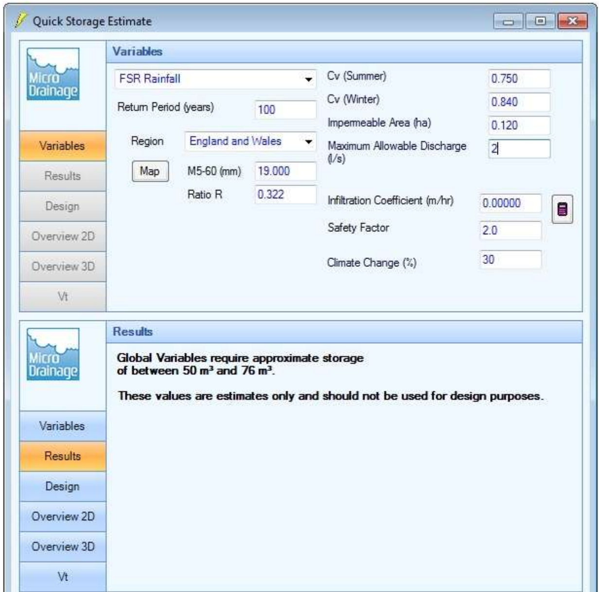
Figure 10. Microdrainage Quick Storage Estimate Attenuation Assessment – Area C School Car Park
