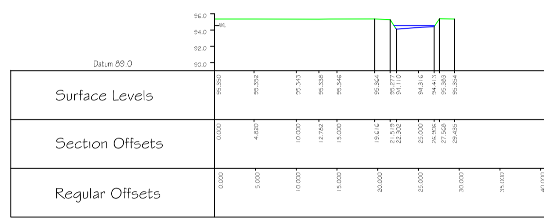
Cross Section 4 HECRAS XS: 40
