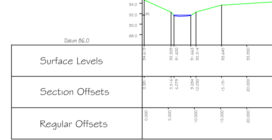
Cross Section 19 HECRAS XS: 25
