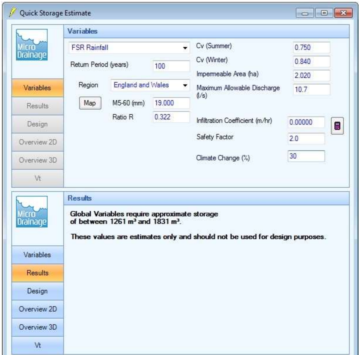
Figure 8. Microdrainage Quick Storage Estimate Attenuation Assessment – Commercial Area A North
