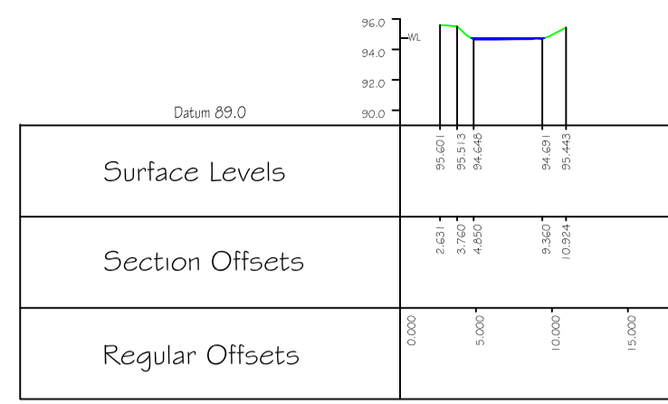
Cross Section 2 HECRAS XS: 42
