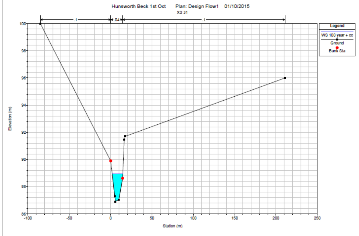
Figure 3.4: Cross Section 13 – 1 in 100 year plus climate change Unobstructed Flow
