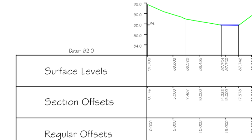
Cross Section 28 HECRAS XS: 16 Vehicle bridge deck - downstream face, facing downstream
