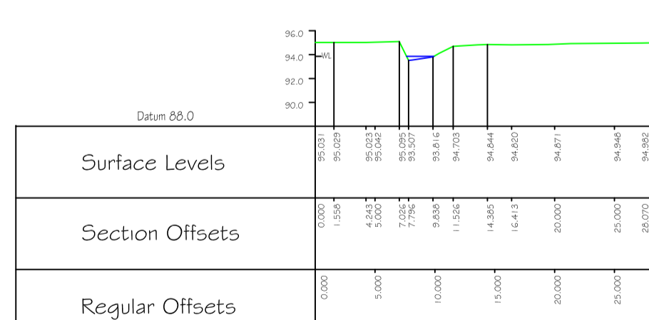
Cross Section 7 HECRAS XS: 37
