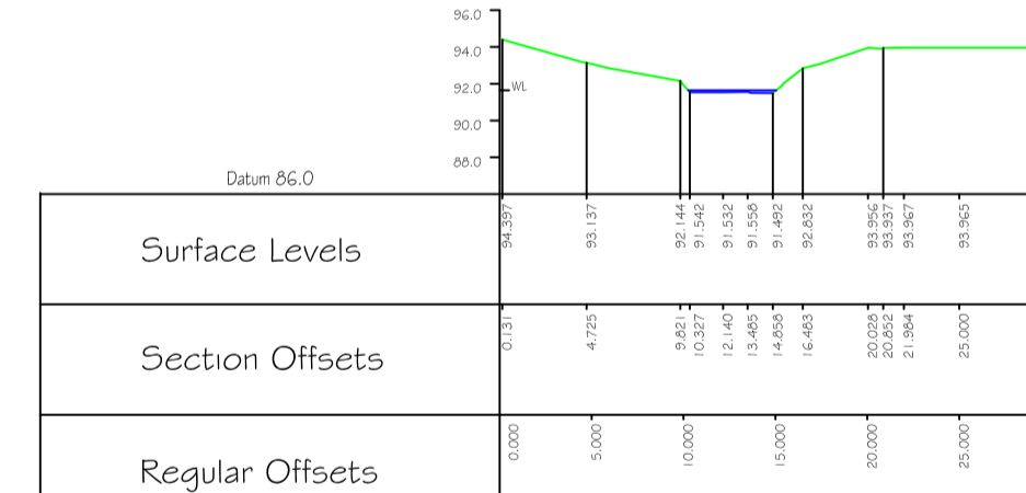
Cross Section 20 HECRAS XS: 24
