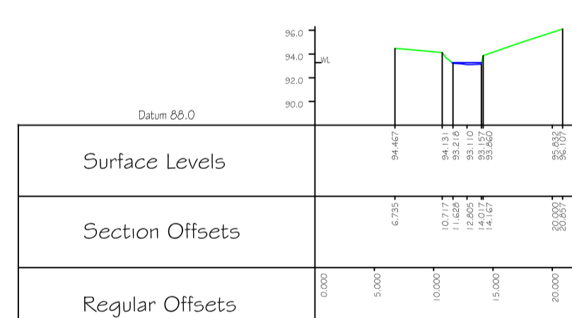
Cross Section 12 HECRAS XS: 32
