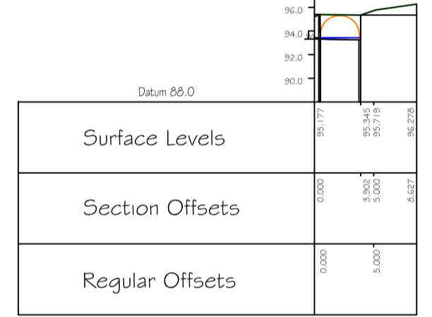
Cross Section 12 HECRAS XS: 32
