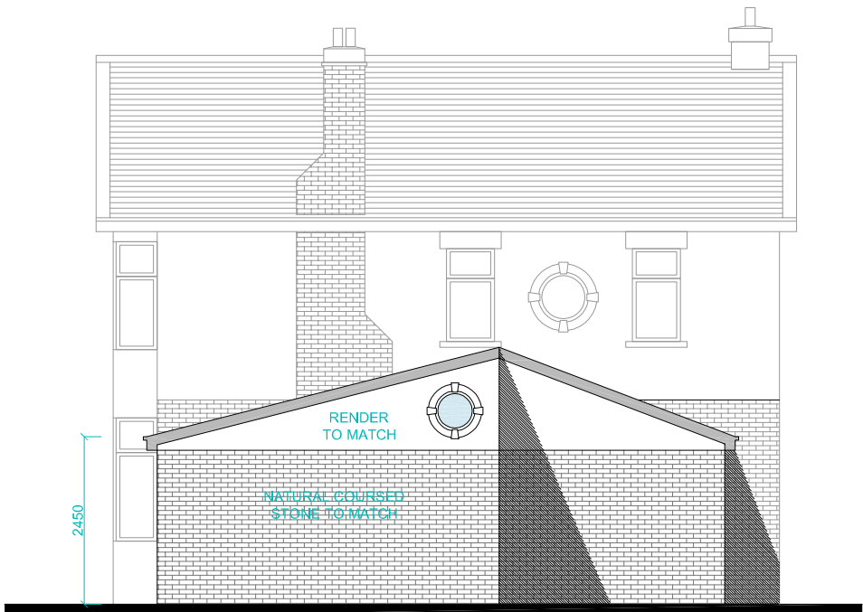
PROPOSED REAR ELEVATION SCALE 1:100@A3
