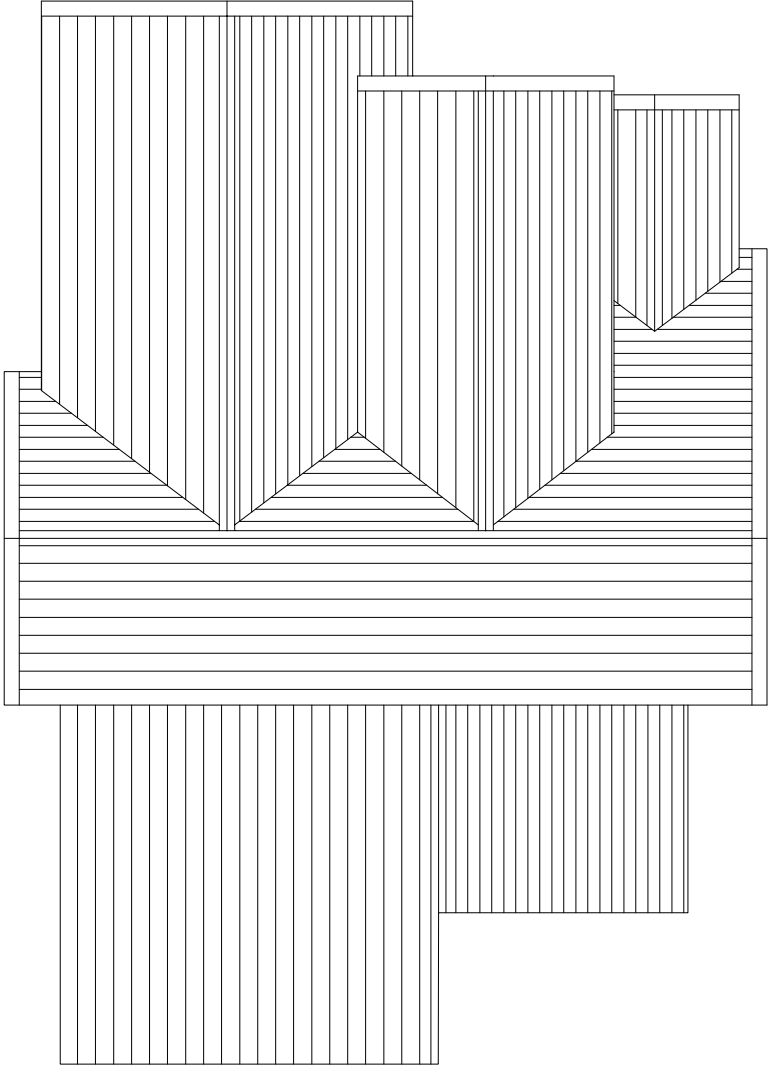
PROPOSED ROOF PLAN SCALE 1:100@A3
