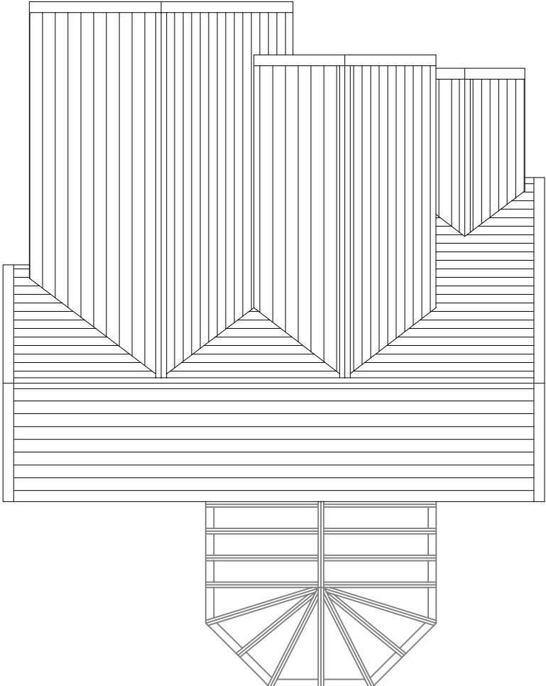
EXISTING ROOF PLAN SCALE 1:100@A3
