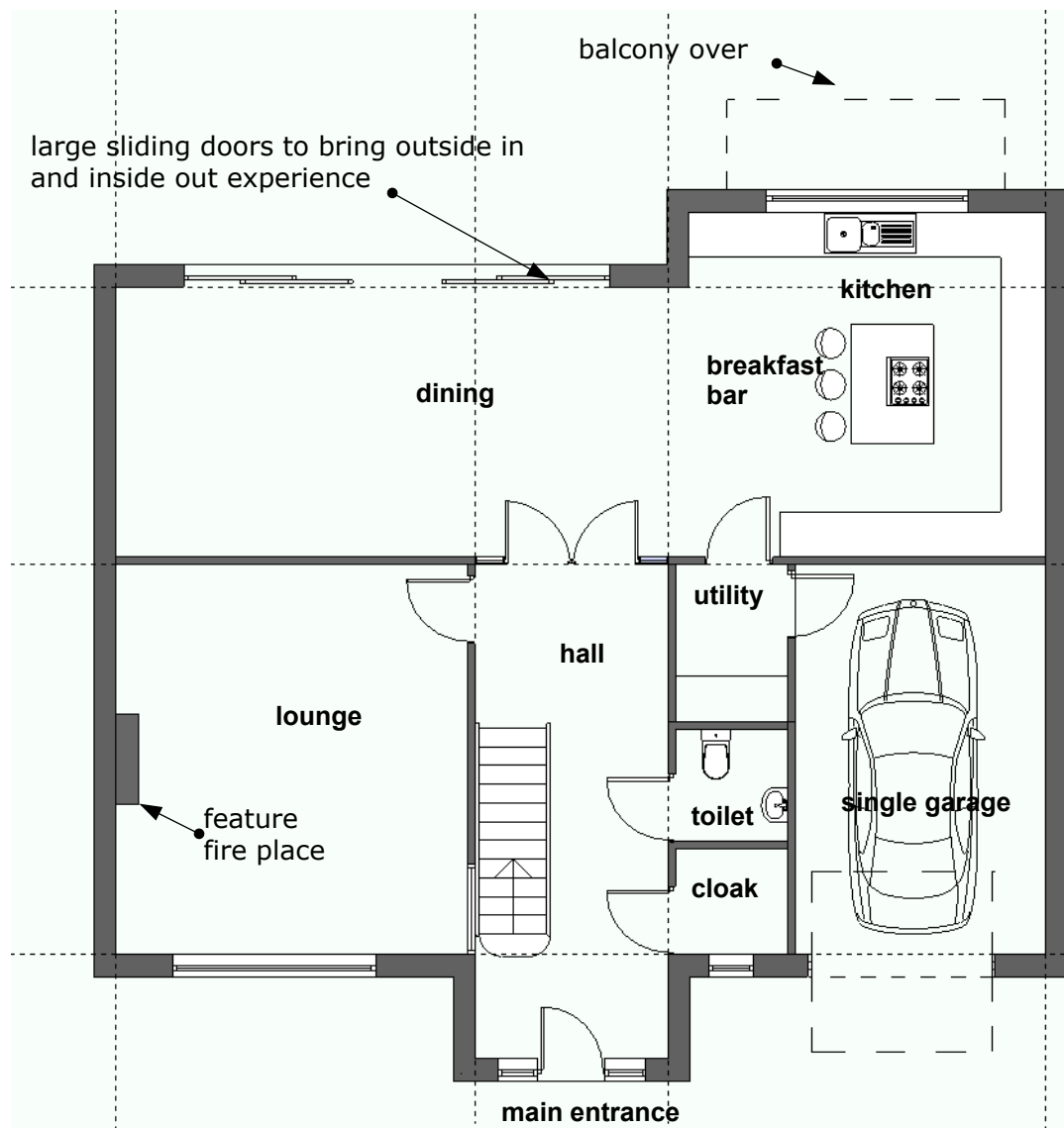
Ground floor as proposed Plot 1
