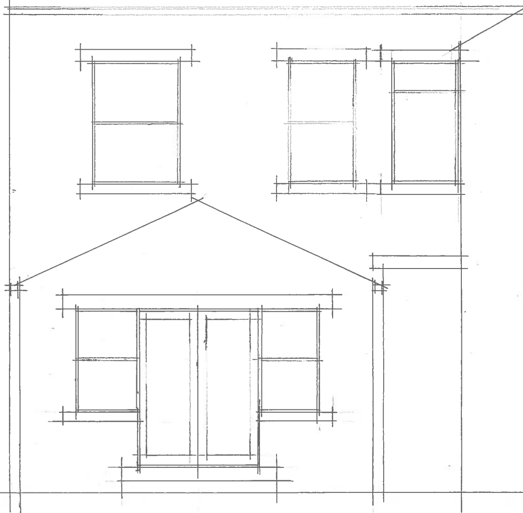
REAR ELEVATION
