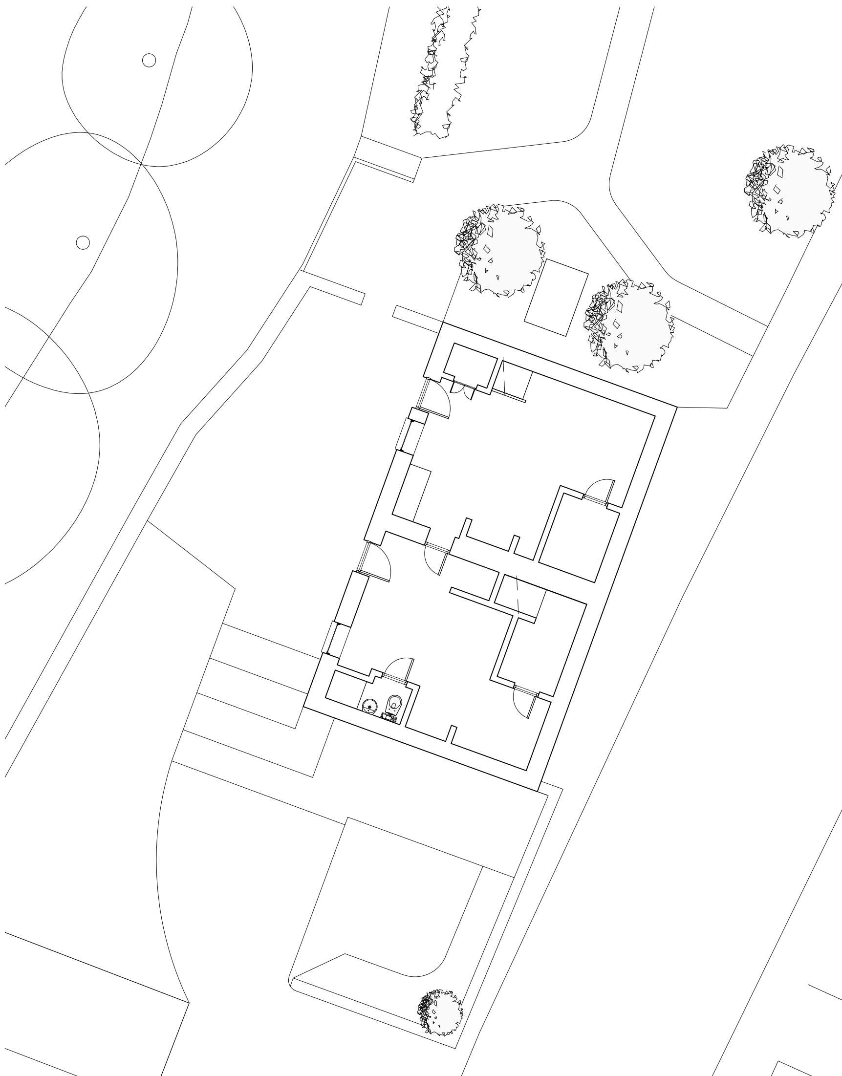
Lower Ground Floor Plan 1:100
