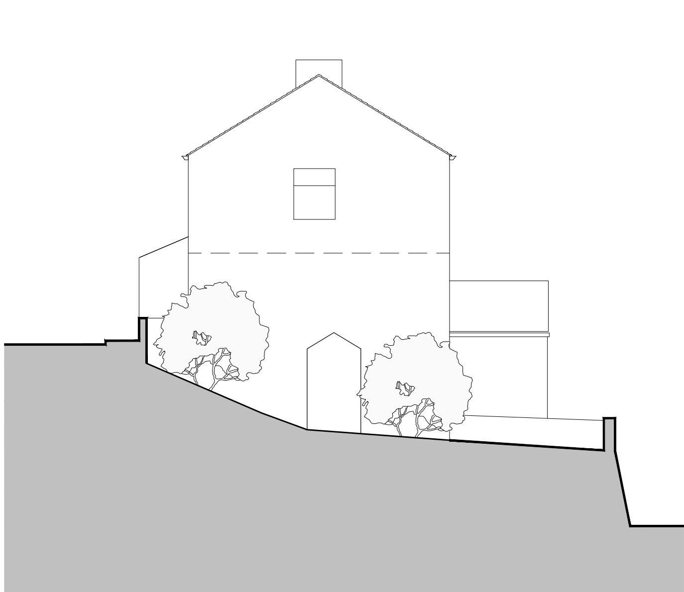
Existing Northern (Garden) Elevation 1:100
