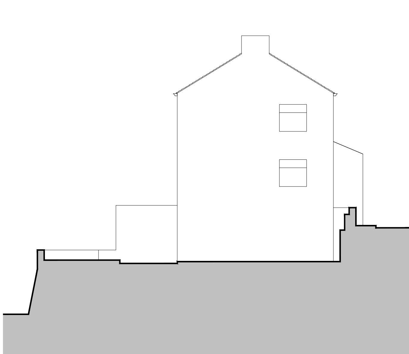
Existing Southern Elevation 1:100
