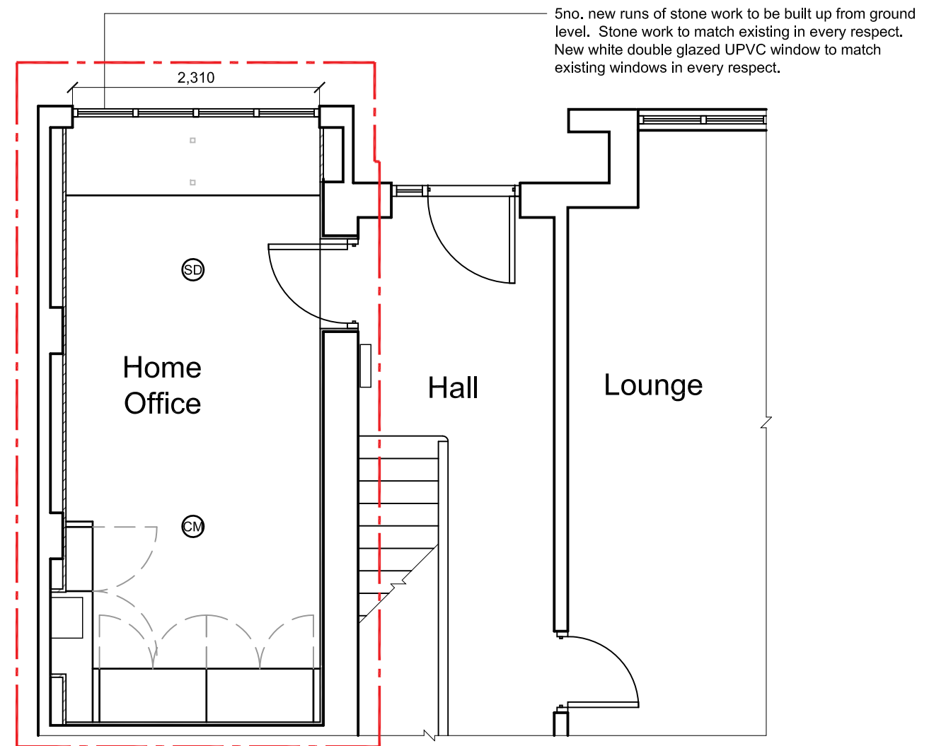
Proposed layout
