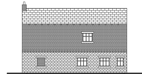
East elevation
