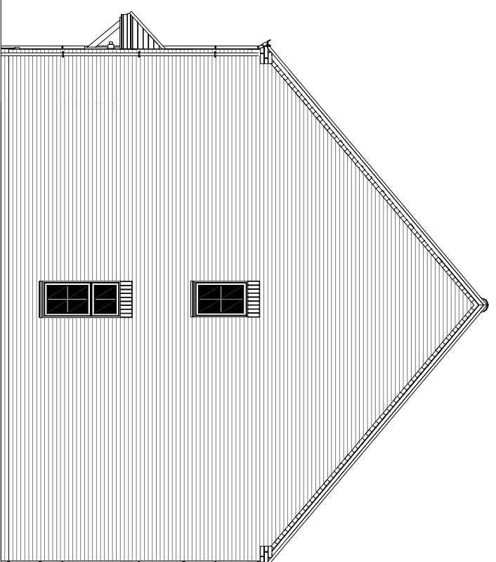
Side Elevation
