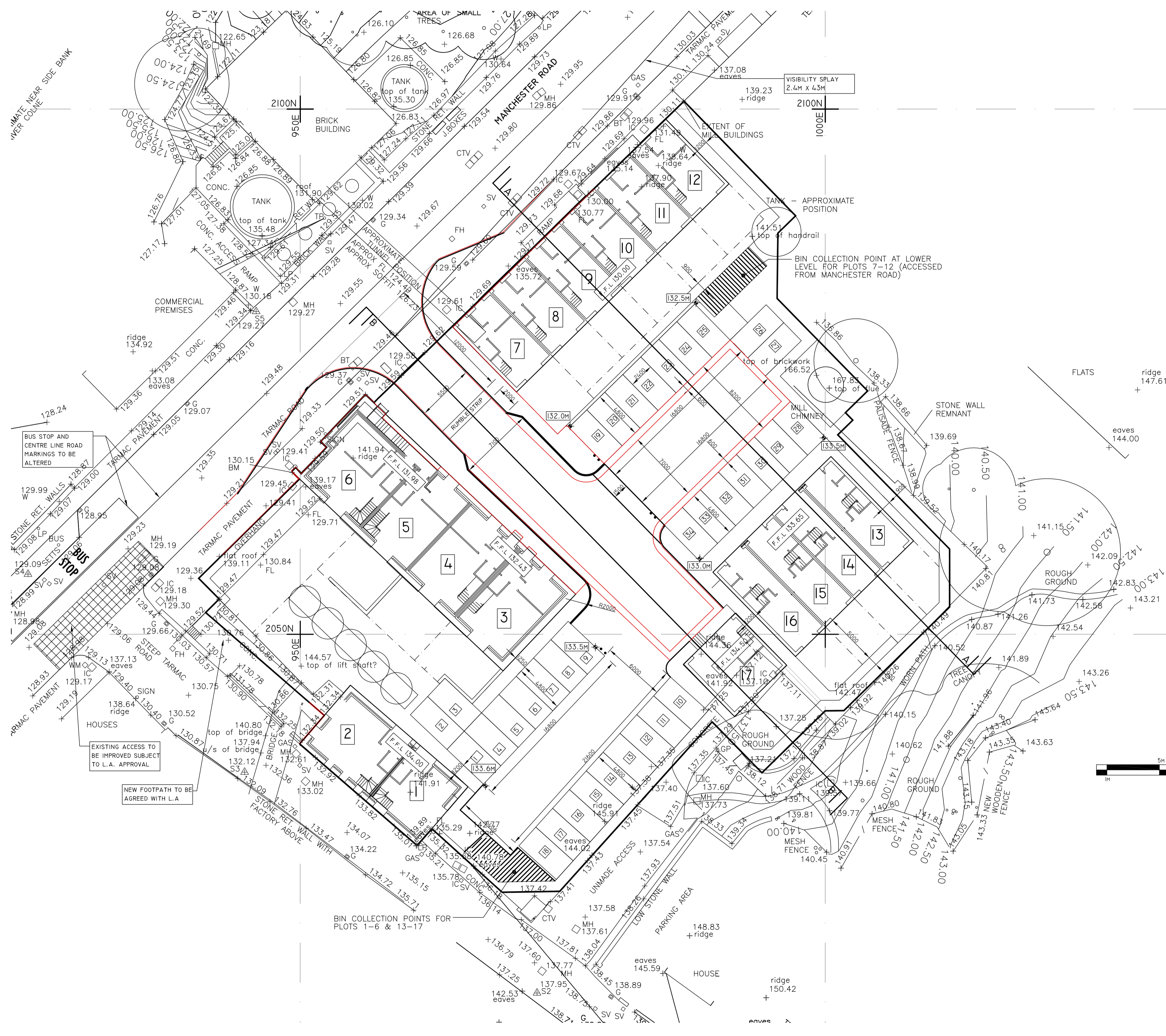
GENERAL ARRANGEMENT OF EXISTING LAYOUT OVERLAID OVER SITE SURVEY 1:200 @ AI
