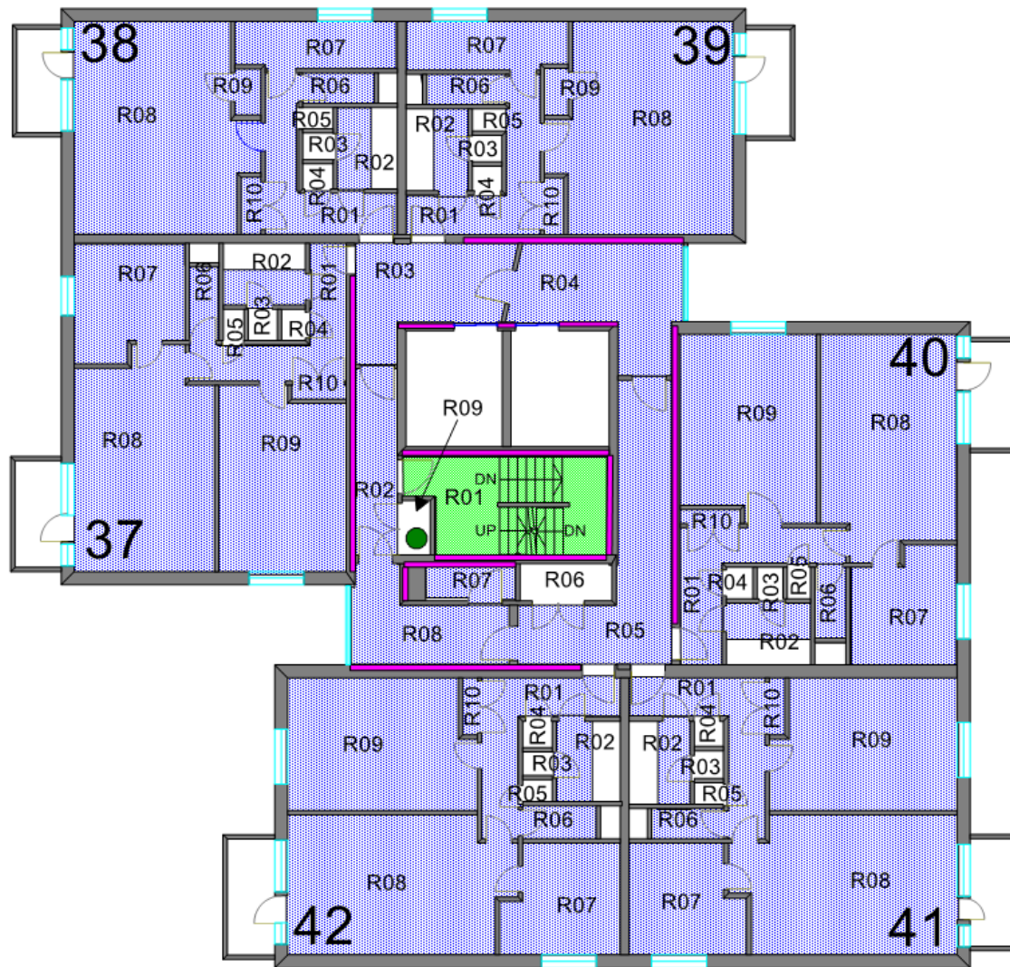
TWELFTH FLOOR
