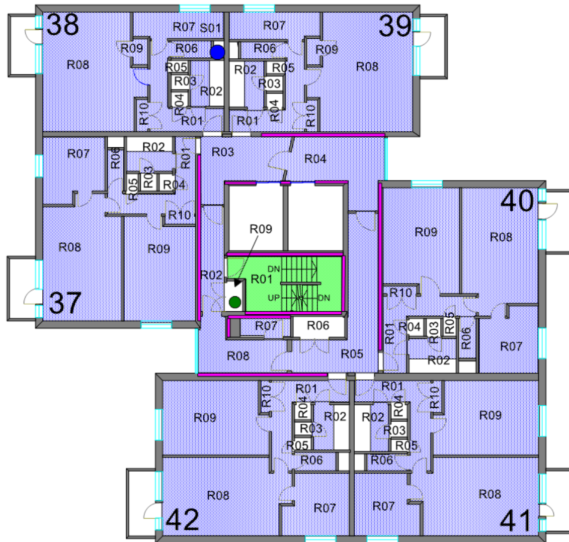
TENTH FLOOR
