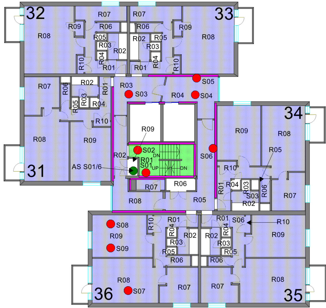
ELEVENTH FLOOR
