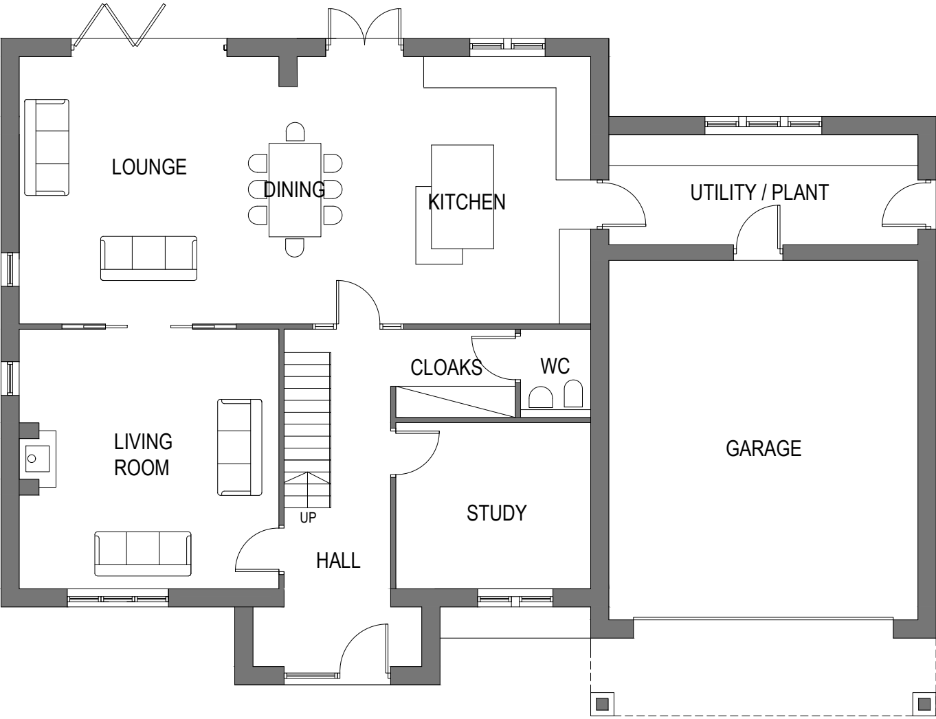
GROUND FLOOR PLAN PLOT 2
