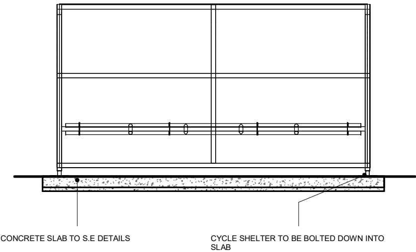
SMOKING SHELTER SECTION A-A 1 : 50
