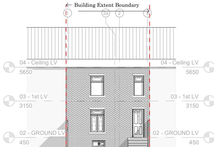
1 Rear Elevation 1 : 100
