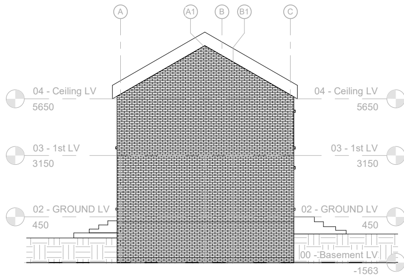
2 Right Side Elevation 1 : 100
