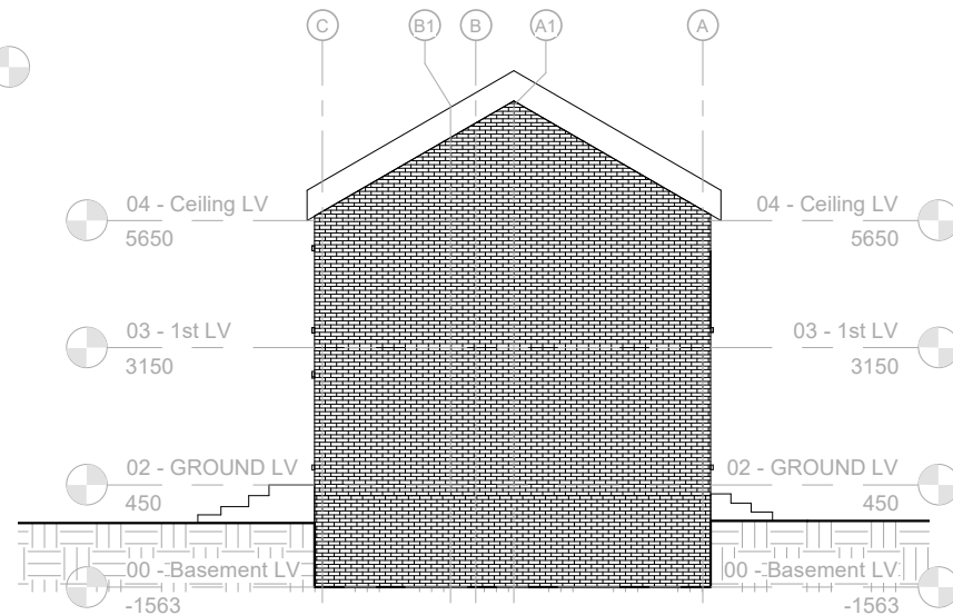
2 Left Side Elevation 1 : 100
