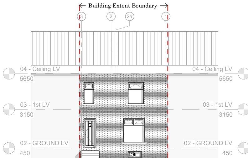
1 Front Elevation 1 : 100
