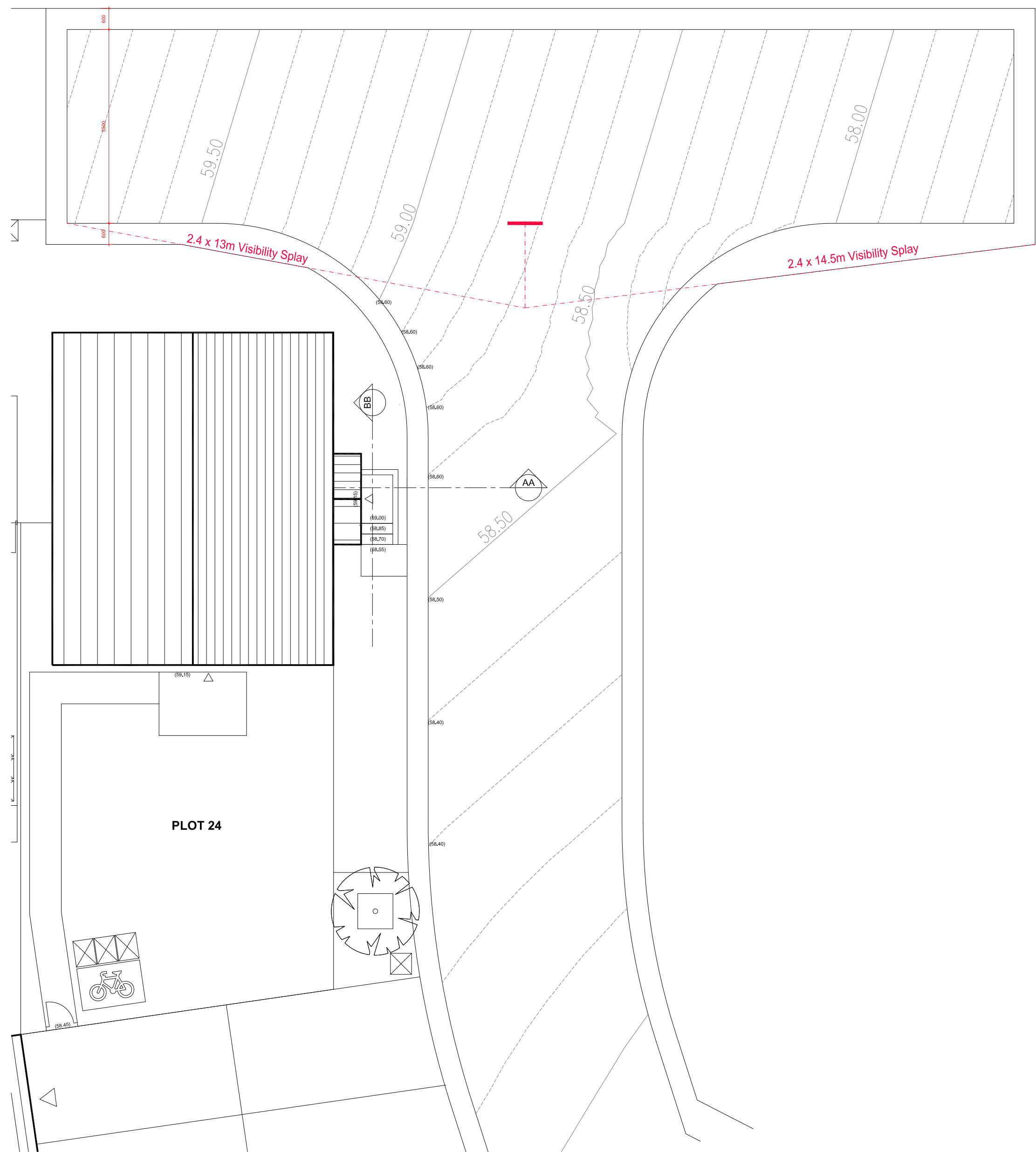
Proposed Plan 1:100
