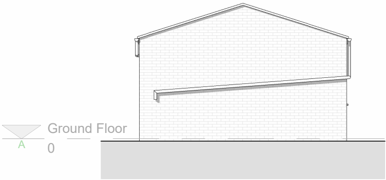
East Elevation - Existing 1 : 100
