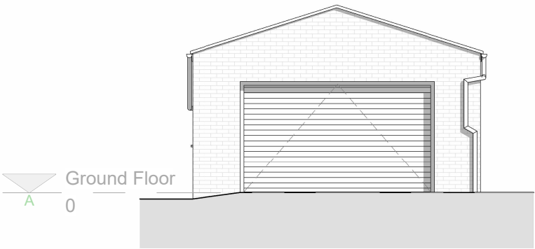
West Elevation - Existing 1 : 100
