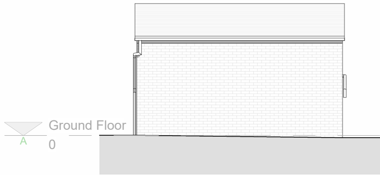
South Elevation - Existing 1 : 100
