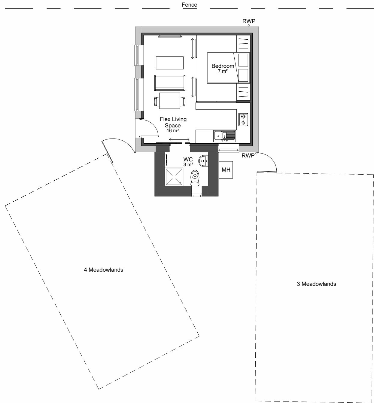
Ground Floor - Proposed 1 : 100
