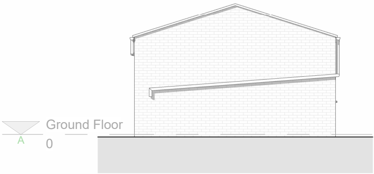
East Elevation - Proposed 1 : 100
