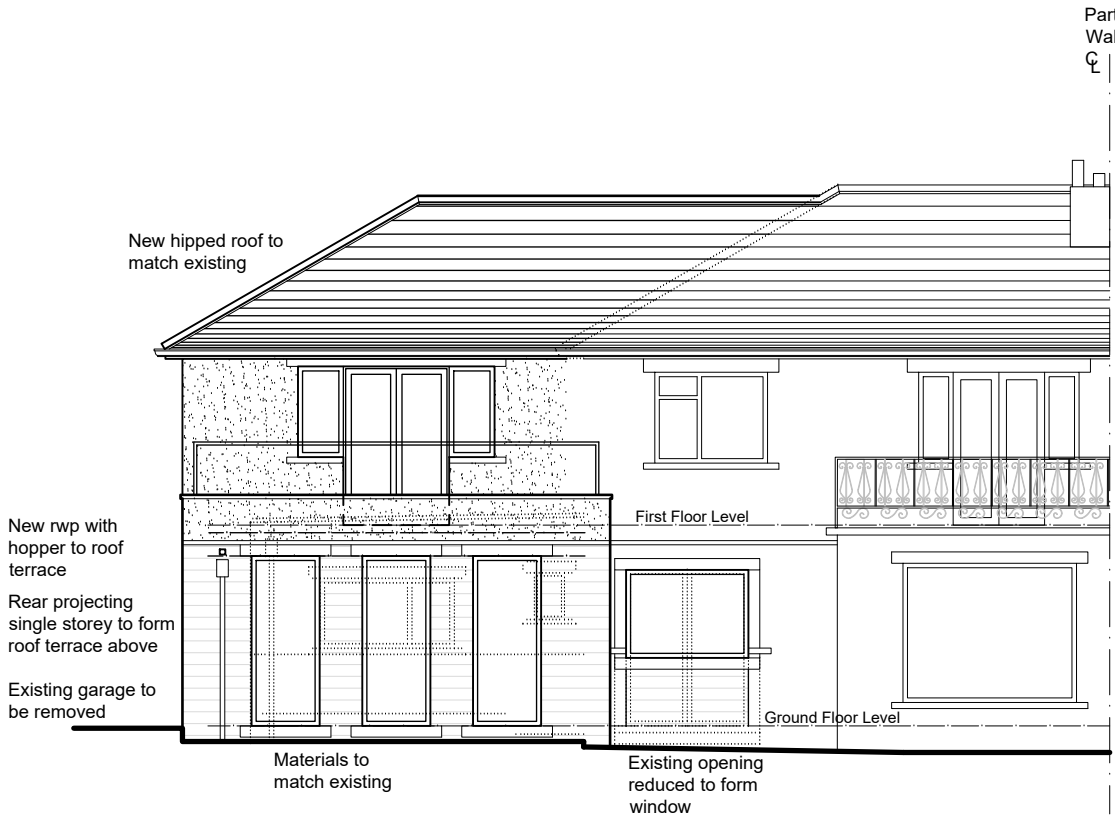
South Elevation (rear)
