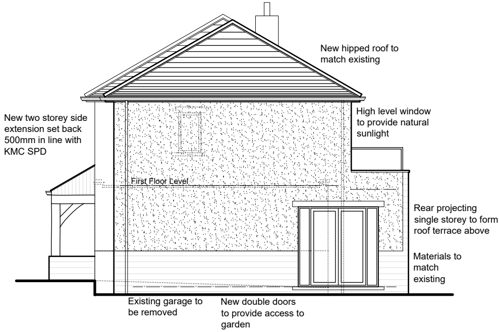
West Elevation (side)
