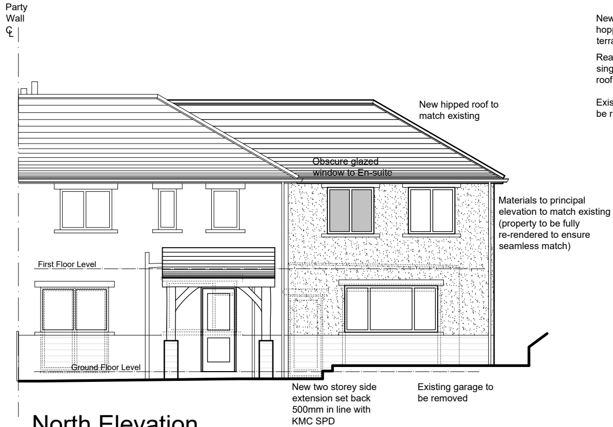
North Elevation (front)
