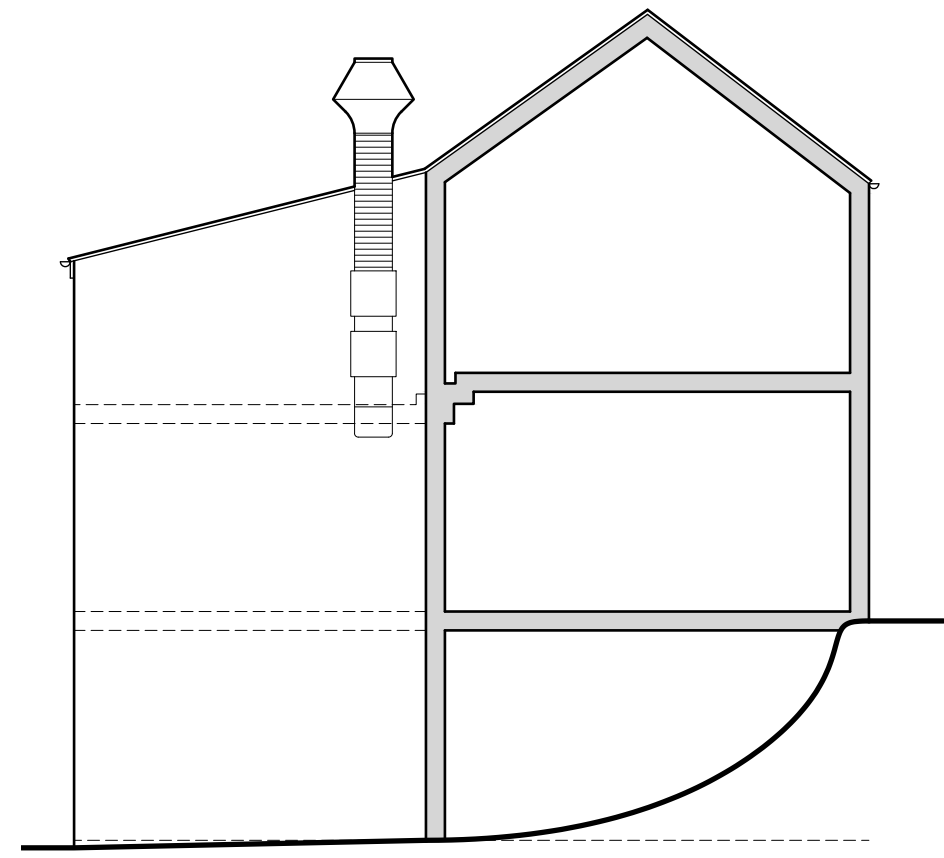
EAST ELEVATION
