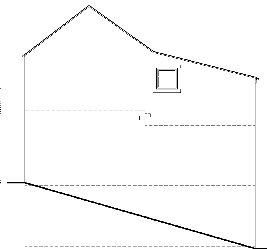
WEST ELEVATION
