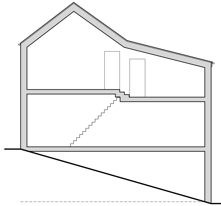
SECTION
