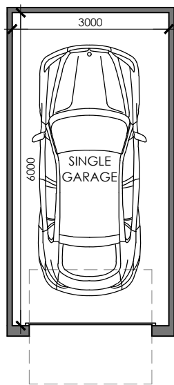
FLOOR PLAN
